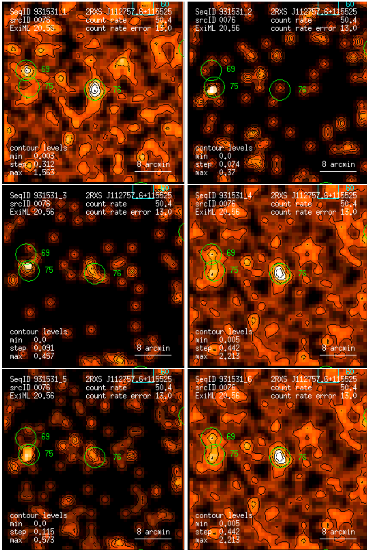
Figure 76: RASS 931531: detection 0076: band rate images, Gaussian filter: (1) PSPC channels 11 – 41, (2) 52 – 90, (3) 91 – 201, (4) 11 – 235, (5) 52 – 201, (6) 11 – 201. Broad band rates in counts/ks. Band rate contour levels in counts/ks/arcmin 2 .
