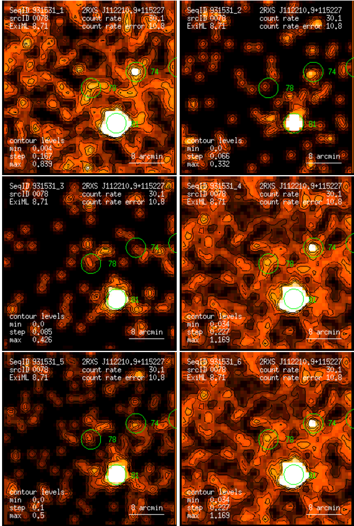
Figure 78: RASS 931531: detection 0078: band rate images, Gaussian filter: (1) PSPC channels 11 – 41, (2) 52 – 90, (3) 91 – 201, (4) 11 – 235, (5) 52 – 201, (6) 11 – 201. Broad band rates in counts/ks. Band rate contour levels in counts/ks/arcmin 2 .
