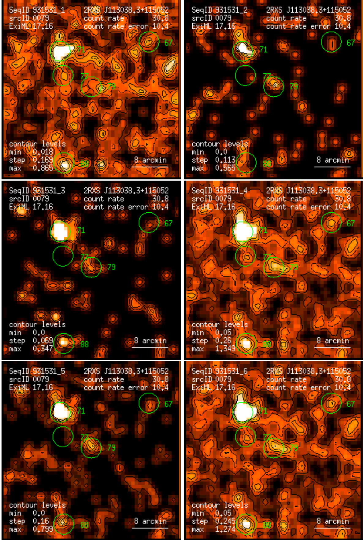
Figure 79: RASS 931531: detection 0079: band rate images, Gaussian filter: (1) PSPC channels 11 – 41, (2) 52 – 90, (3) 91 – 201, (4) 11 – 235, (5) 52 – 201, (6) 11 – 201. Broad band rates in counts/ks. Band rate contour levels in counts/ks/arcmin 2 .
