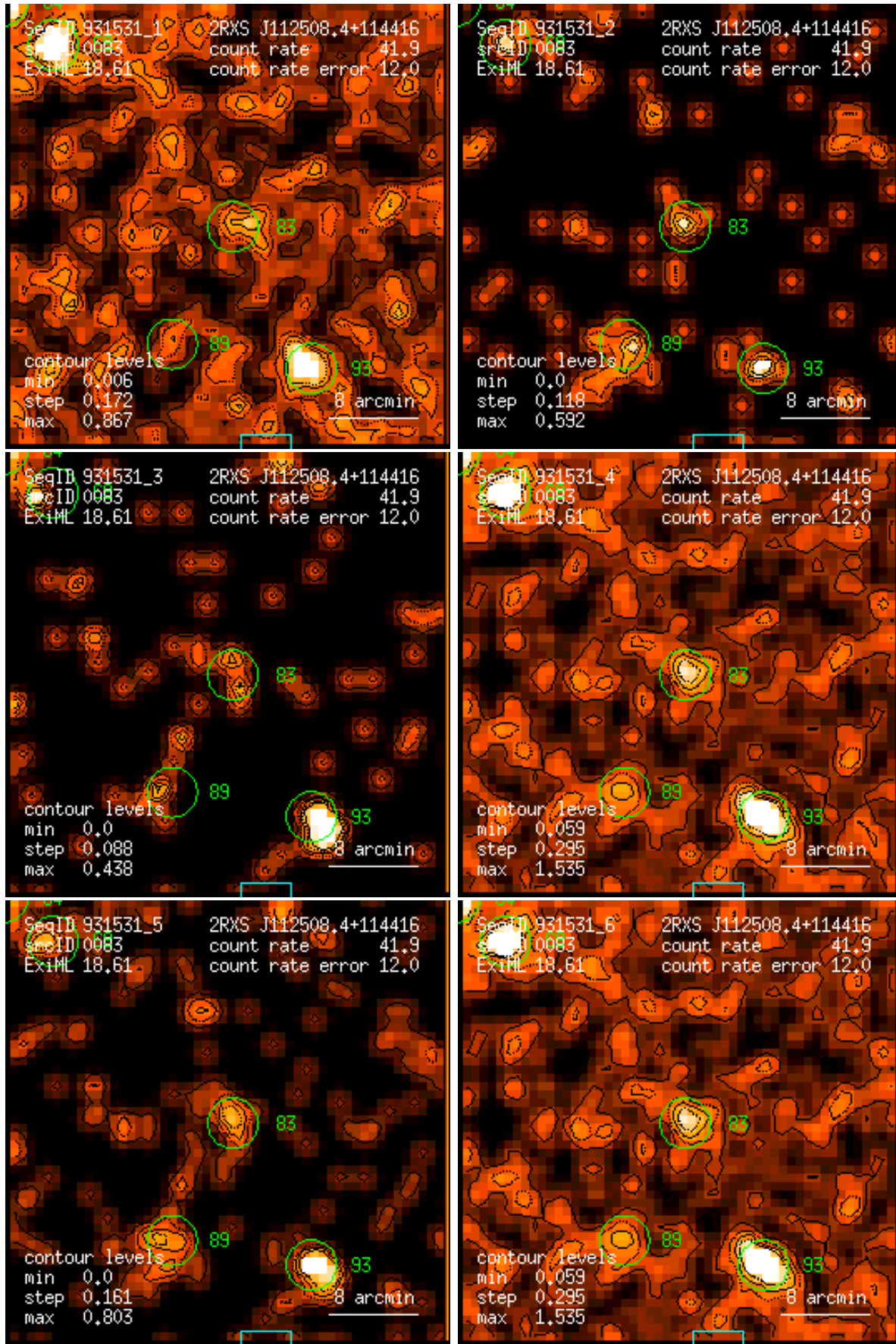
Figure 83: RASS 931531: detection 0083: band rate images, Gaussian filter: (1) PSPC channels 11 – 41, (2) 52 – 90, (3) 91 – 201, (4) 11 – 235, (5) 52 – 201, (6) 11 – 201. Broad band rates in counts/ks. Band rate contour levels in counts/ks/arcmin 2 .
