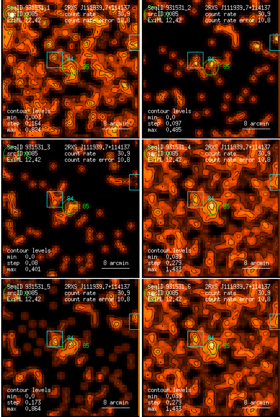
Figure 85: RASS 931531: detection 0085: band rate images, Gaussian filter: (1) PSPC channels 11 – 41, (2) 52 – 90, (3) 91 – 201, (4) 11 – 235, (5) 52 – 201, (6) 11 – 201. Broad band rates in counts/ks. Band rate contour levels in counts/ks/arcmin 2 .
