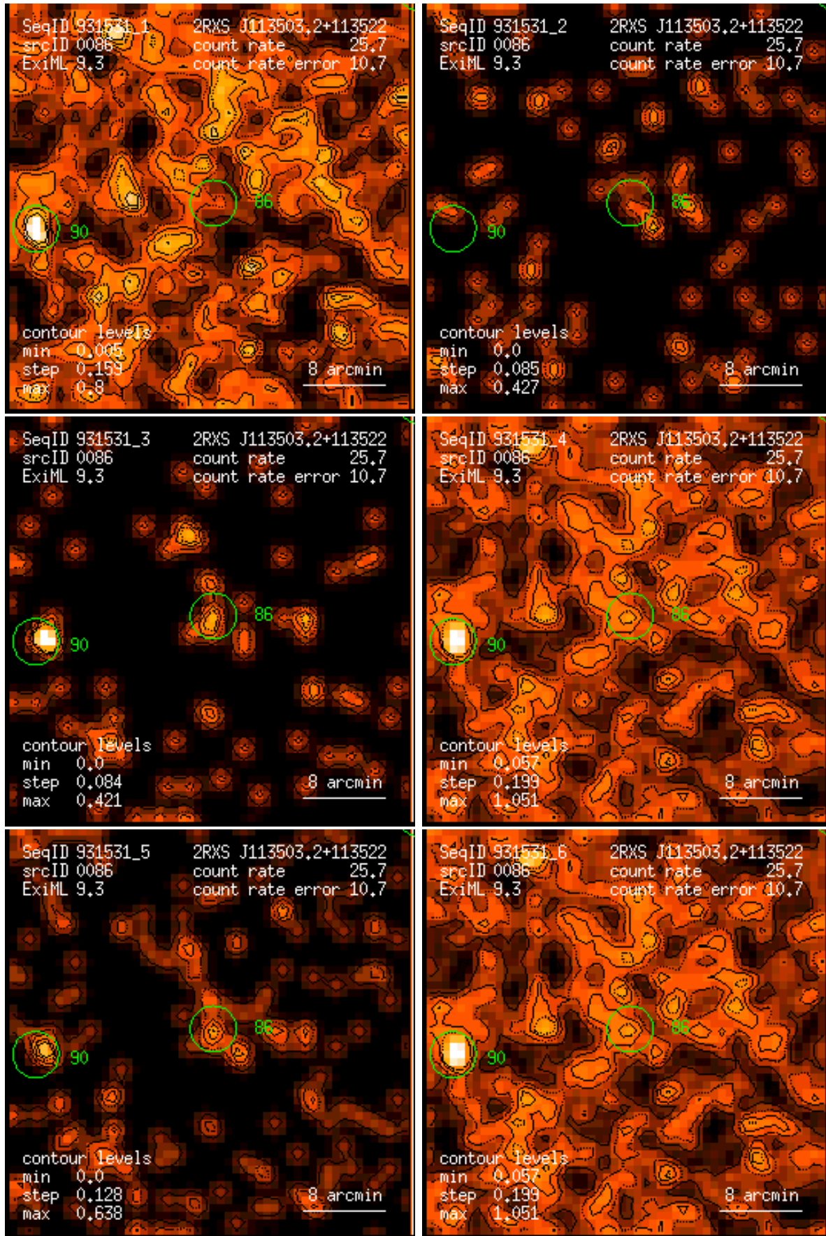
Figure 86: RASS 931531: detection 0086: band rate images, Gaussian filter: (1) PSPC channels 11 – 41, (2) 52 – 90, (3) 91 – 201, (4) 11 – 235, (5) 52 – 201, (6) 11 – 201. Broad band rates in counts/ks. Band rate contour levels in counts/ks/arcmin 2 .
