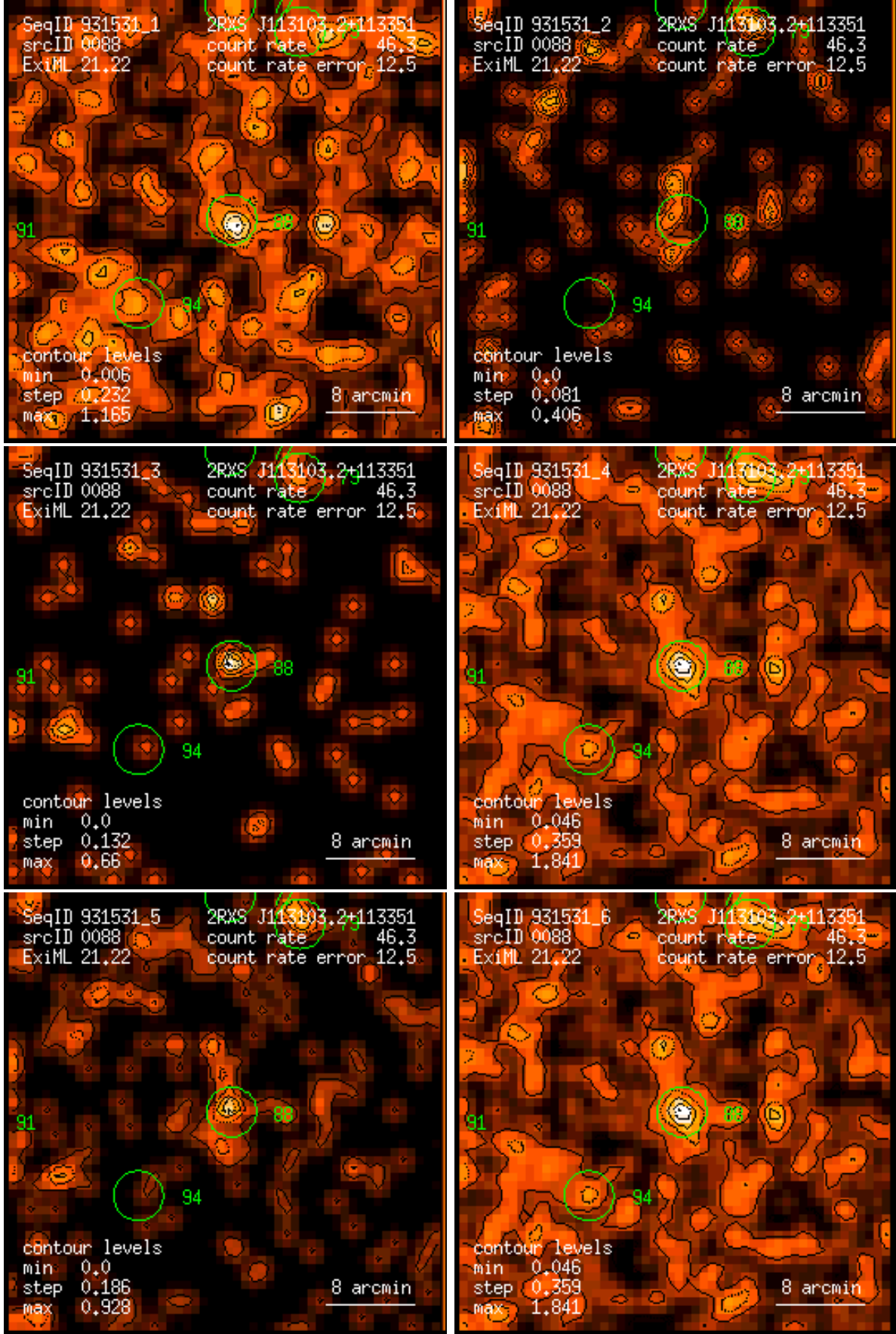
Figure 88: RASS 931531: detection 0088: band rate images, Gaussian filter: (1) PSPC channels 11 – 41, (2) 52 – 90, (3) 91 – 201, (4) 11 – 235, (5) 52 – 201, (6) 11 – 201. Broad band rates in counts/ks. Band rate contour levels in counts/ks/arcmin 2 .
