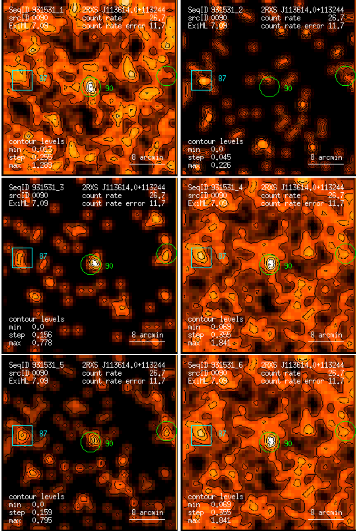
Figure 90: RASS 931531: detection 0090: band rate images, Gaussian filter: (1) PSPC channels 11 – 41, (2) 52 – 90, (3) 91 – 201, (4) 11 – 235, (5) 52 – 201, (6) 11 – 201. Broad band rates in counts/ks. Band rate contour levels in counts/ks/arcmin 2 .
