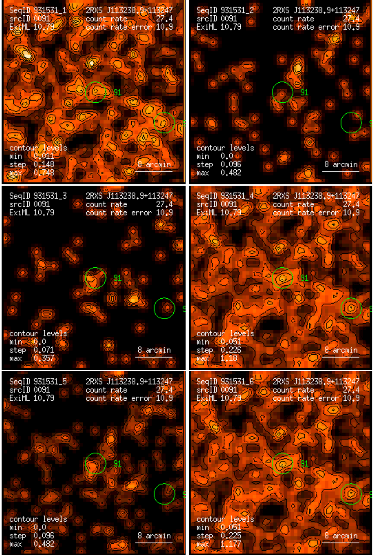
Figure 91: RASS 931531: detection 0091: band rate images, Gaussian filter: (1) PSPC channels 11 – 41, (2) 52 – 90, (3) 91 – 201, (4) 11 – 235, (5) 52 – 201, (6) 11 – 201. Broad band rates in counts/ks. Band rate contour levels in counts/ks/arcmin 2 .
