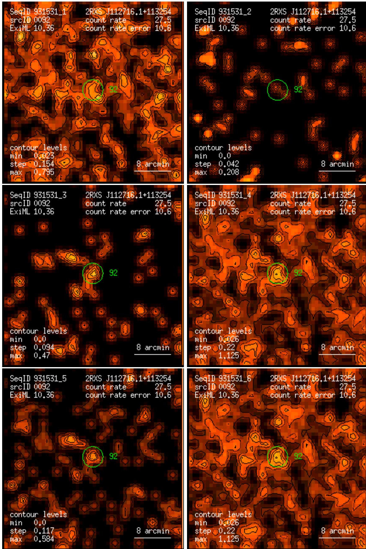
Figure 92: RASS 931531: detection 0092: band rate images, Gaussian filter: (1) PSPC channels 11 – 41, (2) 52 – 90, (3) 91 – 201, (4) 11 – 235, (5) 52 – 201, (6) 11 – 201. Broad band rates in counts/ks. Band rate contour levels in counts/ks/arcmin 2 .
