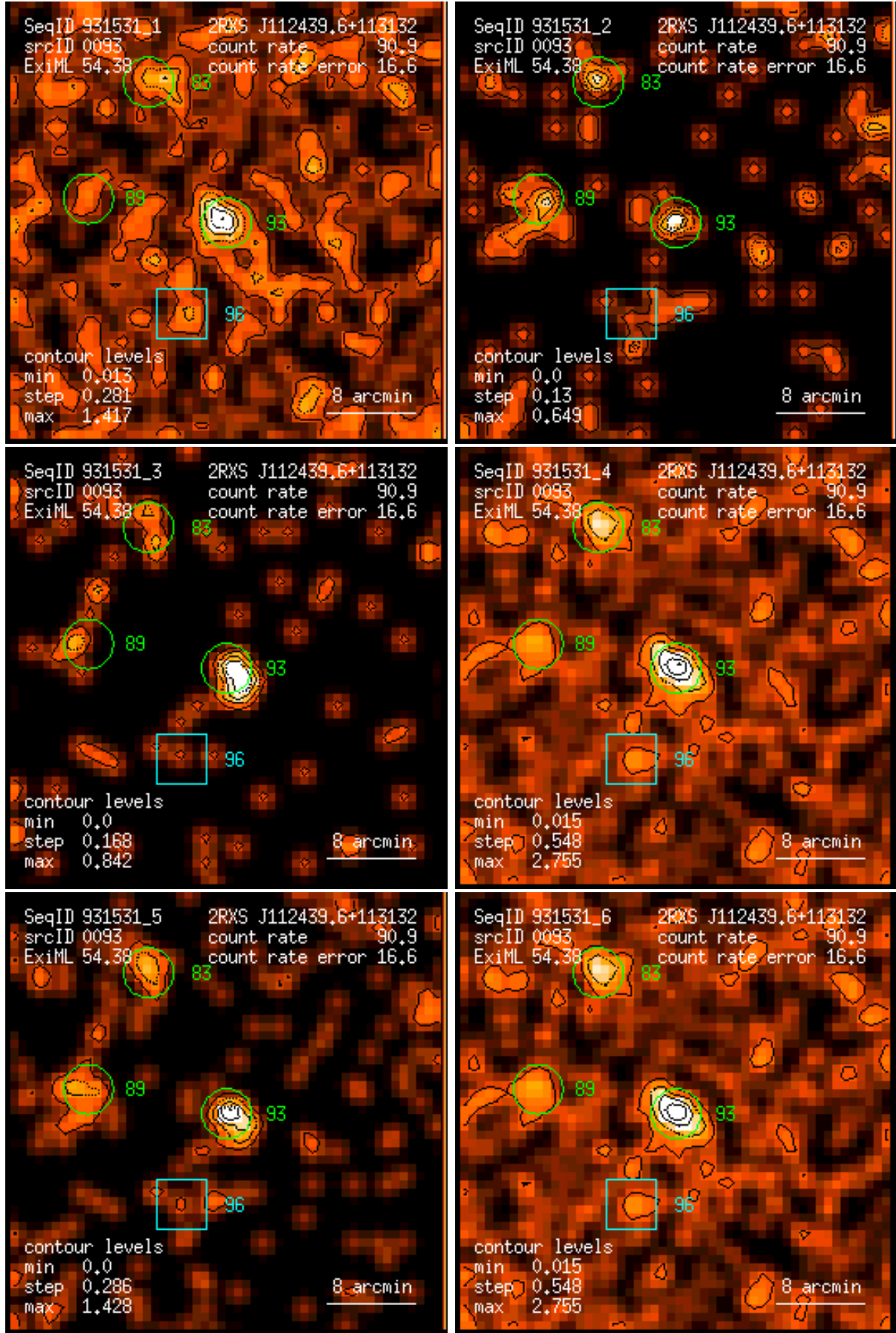
Figure 93: RASS 931531: detection 0093: band rate images, Gaussian filter: (1) PSPC channels 11 – 41, (2) 52 – 90, (3) 91 – 201, (4) 11 – 235, (5) 52 – 201, (6) 11 – 201. Broad band rates in counts/ks. Band rate contour levels in counts/ks/arcmin 2 .
