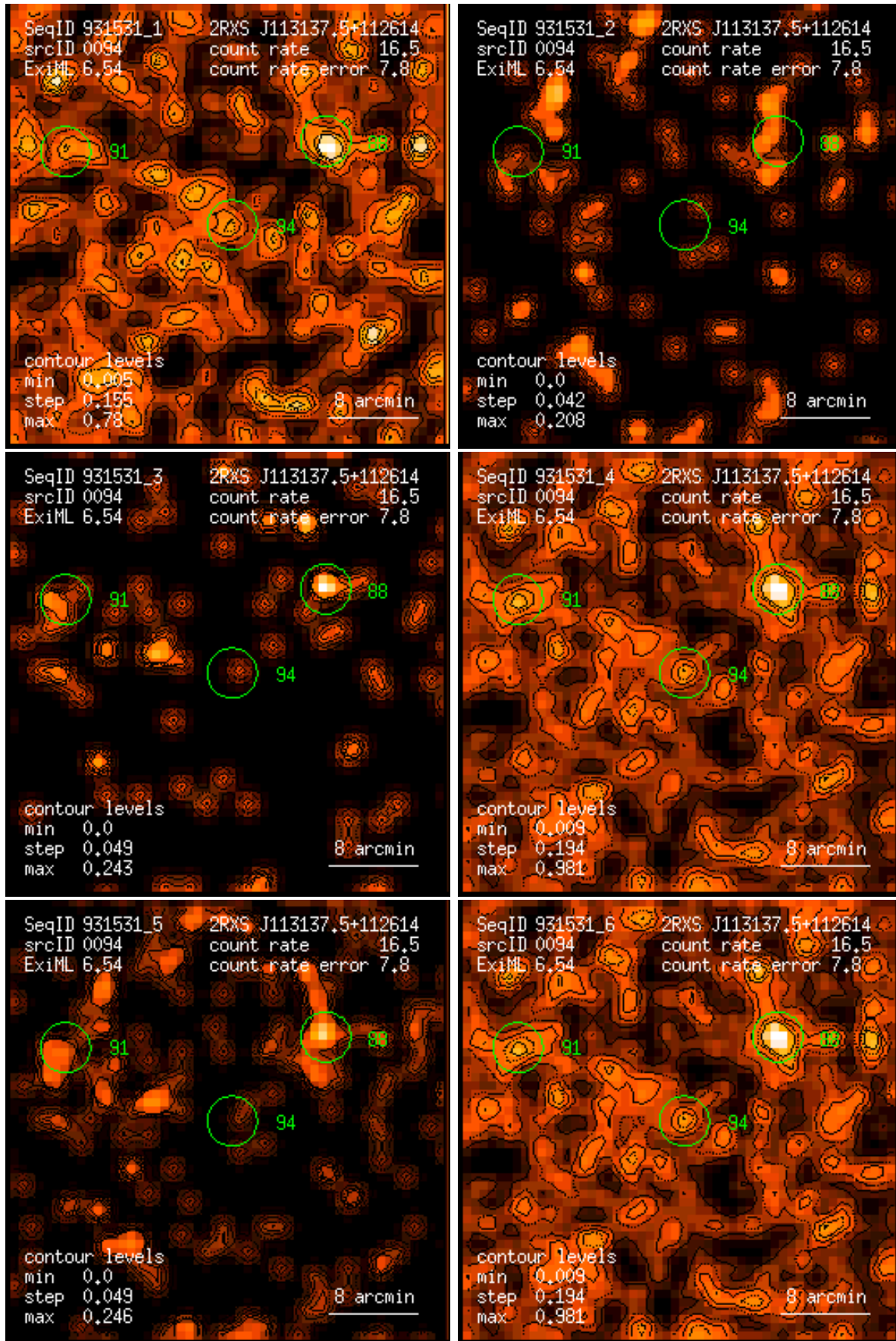
Figure 94: RASS 931531: detection 0094: band rate images, Gaussian filter: (1) PSPC channels 11 – 41, (2) 52 – 90, (3) 91 – 201, (4) 11 – 235, (5) 52 – 201, (6) 11 – 201. Broad band rates in counts/ks. Band rate contour levels in counts/ks/arcmin 2 .
