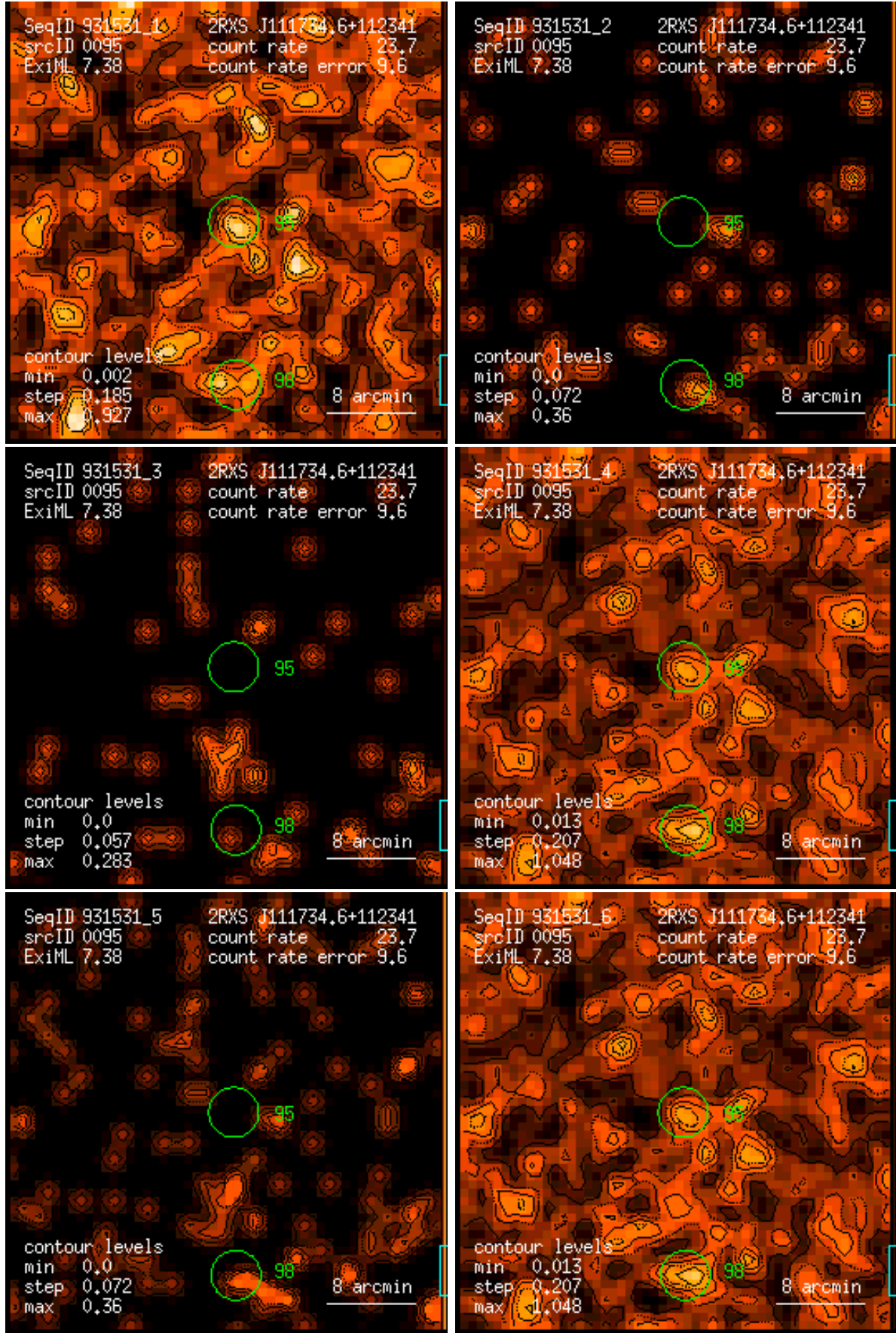
Figure 95: RASS 931531: detection 0095: band rate images, Gaussian filter: (1) PSPC channels 11 – 41, (2) 52 – 90, (3) 91 – 201, (4) 11 – 235, (5) 52 – 201, (6) 11 – 201. Broad band rates in counts/ks. Band rate contour levels in counts/ks/arcmin 2 .
