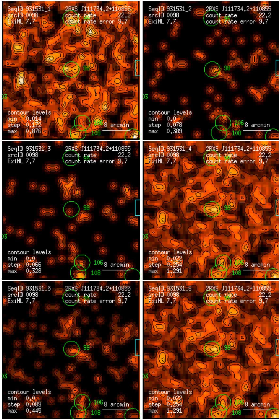
Figure 98: RASS 931531: detection 0098: band rate images, Gaussian filter: (1) PSPC channels 11 – 41, (2) 52 – 90, (3) 91 – 201, (4) 11 – 235, (5) 52 – 201, (6) 11 – 201. Broad band rates in counts/ks. Band rate contour levels in counts/ks/arcmin 2 .
