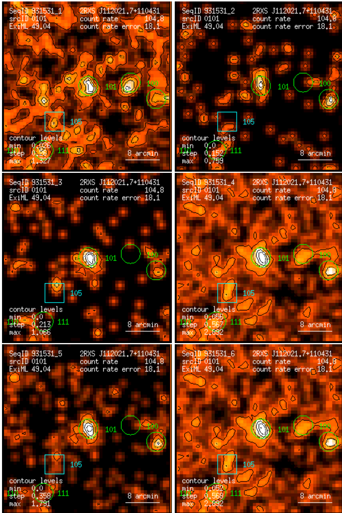
Figure 101: RASS 931531: detection 0101: band rate images, Gaussian filter: (1) PSPC channels 11 – 41, (2) 52 – 90, (3) 91 – 201, (4) 11 – 235, (5) 52 – 201, (6) 11 – 201. Broad band rates in counts/ks. Band rate contour levels in counts/ks/arcmin 2 .
