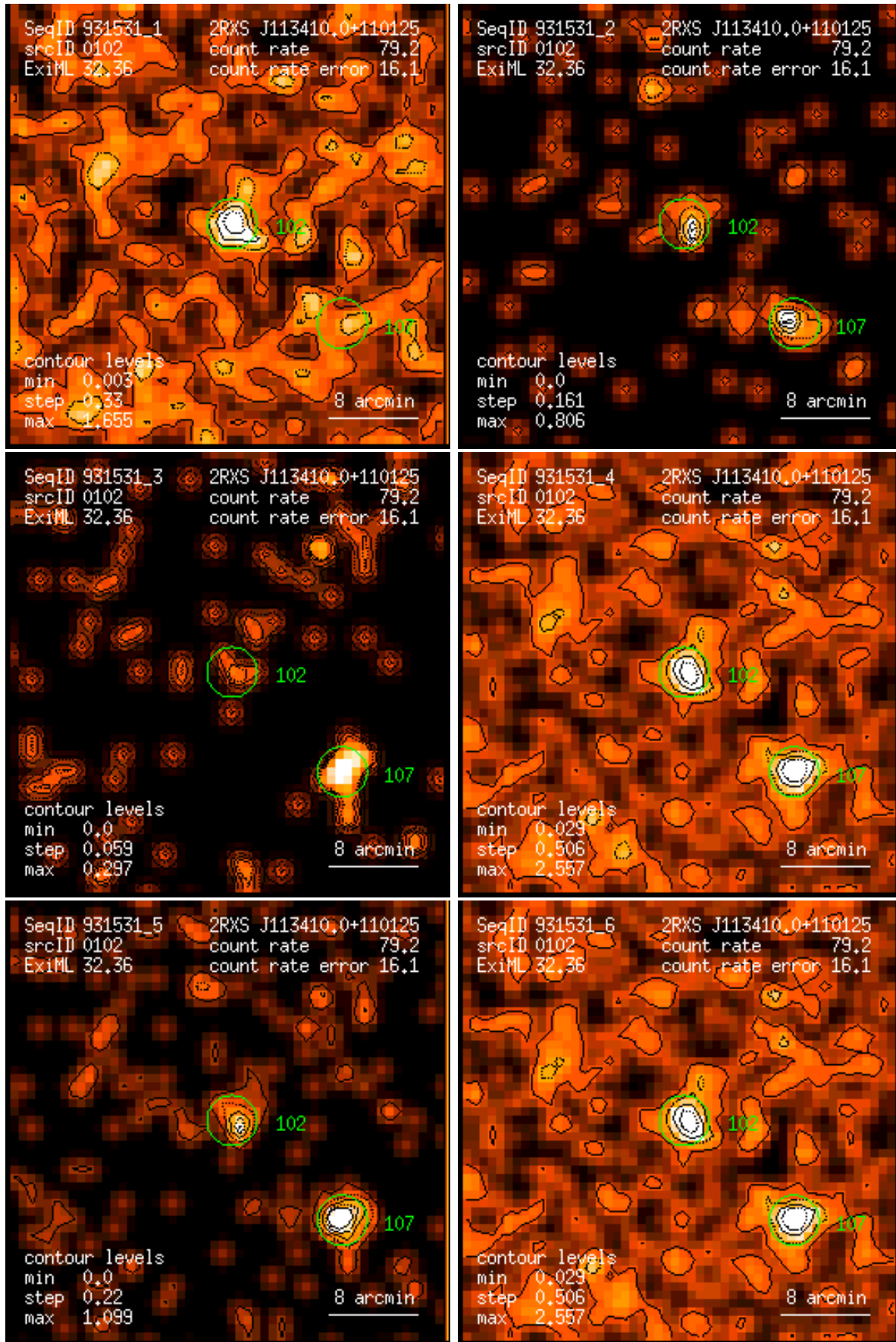
Figure 102: RASS 931531: detection 0102: band rate images, Gaussian filter: (1) PSPC channels 11 – 41, (2) 52 – 90, (3) 91 – 201, (4) 11 – 235, (5) 52 – 201, (6) 11 – 201. Broad band rates in counts/ks. Band rate contour levels in counts/ks/arcmin 2 .
