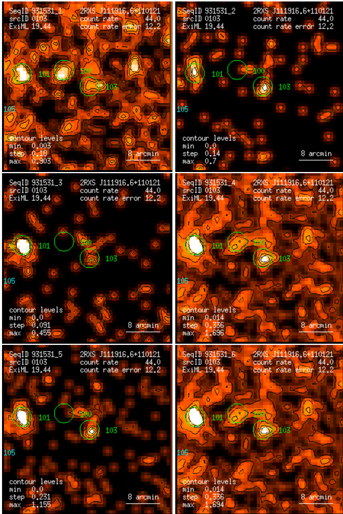
Figure 103: RASS 931531: detection 0103: band rate images, Gaussian filter: (1) PSPC channels 11 – 41, (2) 52 – 90, (3) 91 – 201, (4) 11 – 235, (5) 52 – 201, (6) 11 – 201. Broad band rates in counts/ks. Band rate contour levels in counts/ks/arcmin 2 .
