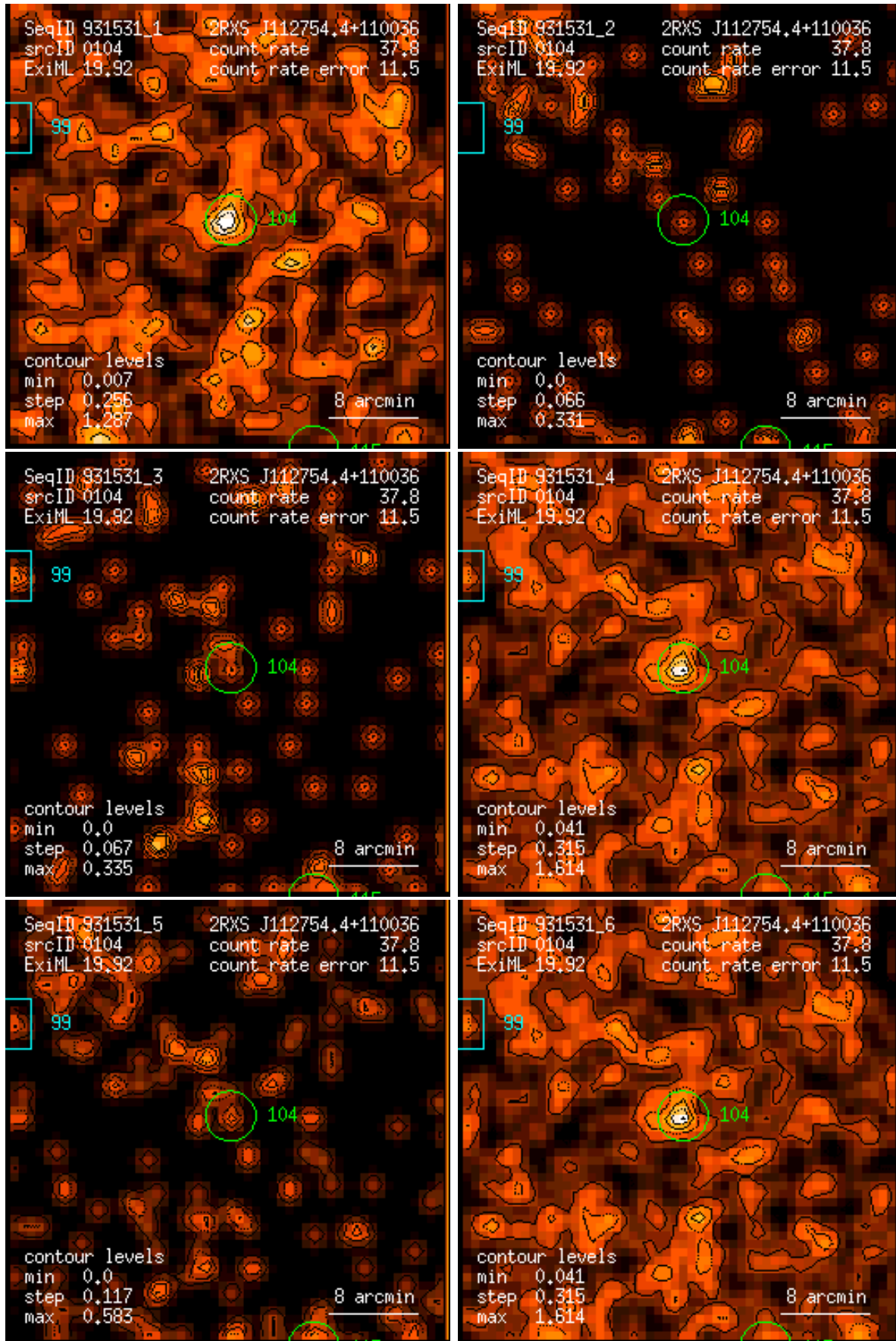
Figure 104: RASS 931531: detection 0104: band rate images, Gaussian filter: (1) PSPC channels 11 – 41, (2) 52 – 90, (3) 91 – 201, (4) 11 – 235, (5) 52 – 201, (6) 11 – 201. Broad band rates in counts/ks. Band rate contour levels in counts/ks/arcmin 2 .
