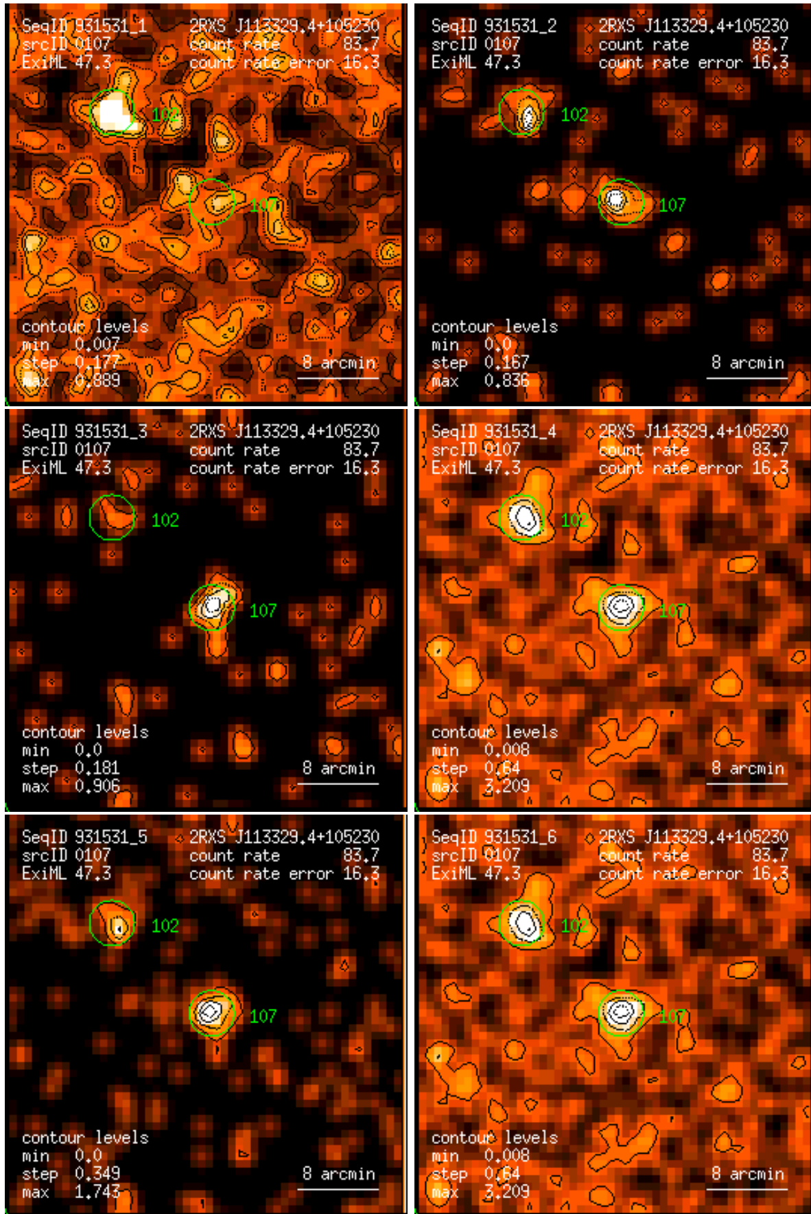
Figure 107: RASS 931531: detection 0107: band rate images, Gaussian filter: (1) PSPC channels 11 – 41, (2) 52 – 90, (3) 91 – 201, (4) 11 – 235, (5) 52 – 201, (6) 11 – 201. Broad band rates in counts/ks. Band rate contour levels in counts/ks/arcmin 2 .
