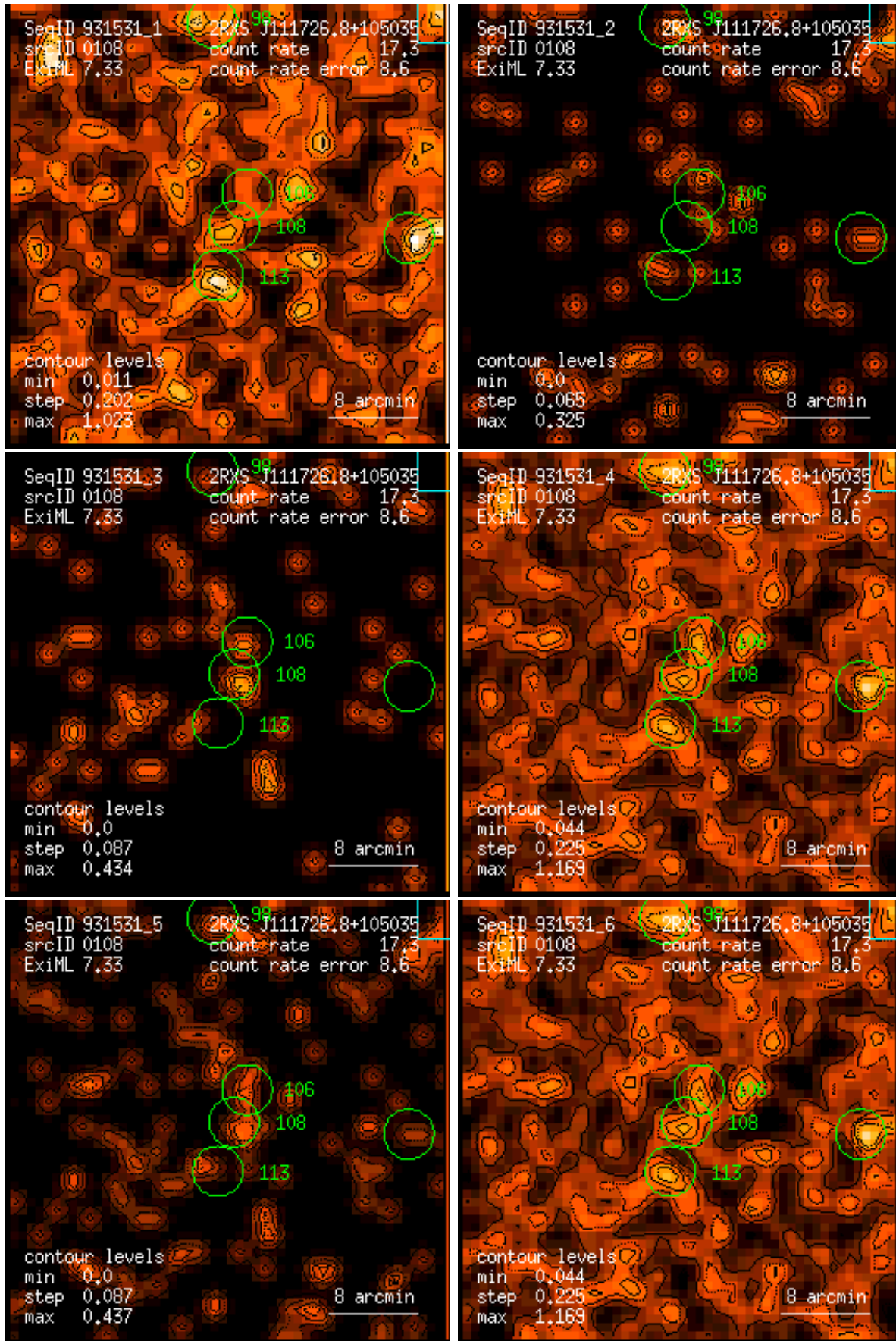
Figure 108: RASS 931531: detection 0108: band rate images, Gaussian filter: (1) PSPC channels 11 – 41, (2) 52 – 90, (3) 91 – 201, (4) 11 – 235, (5) 52 – 201, (6) 11 – 201. Broad band rates in counts/ks. Band rate contour levels in counts/ks/arcmin 2 .
