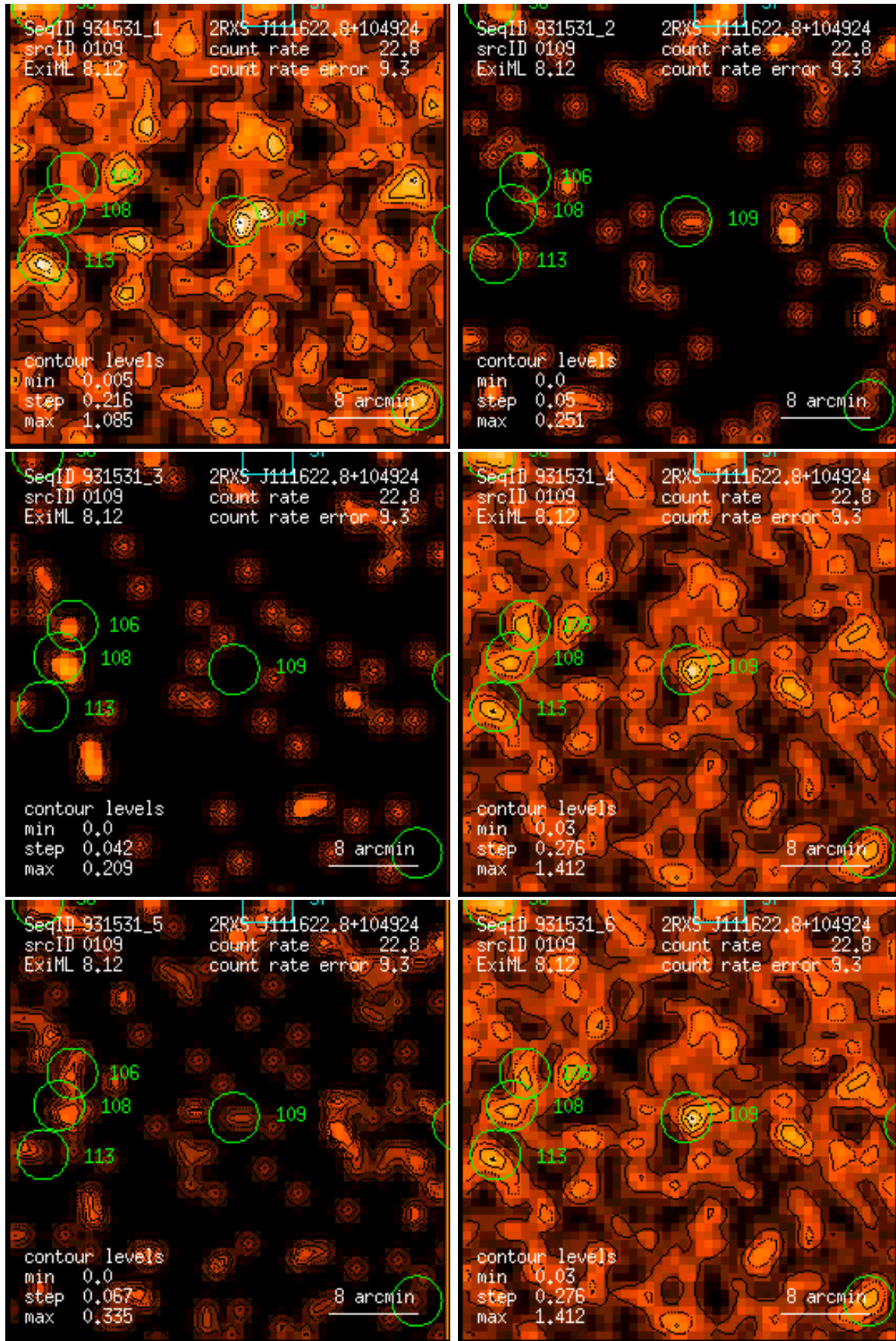
Figure 109: RASS 931531: detection 0109: band rate images, Gaussian filter: (1) PSPC channels 11 – 41, (2) 52 – 90, (3) 91 – 201, (4) 11 – 235, (5) 52 – 201, (6) 11 – 201. Broad band rates in counts/ks. Band rate contour levels in counts/ks/arcmin 2 .
