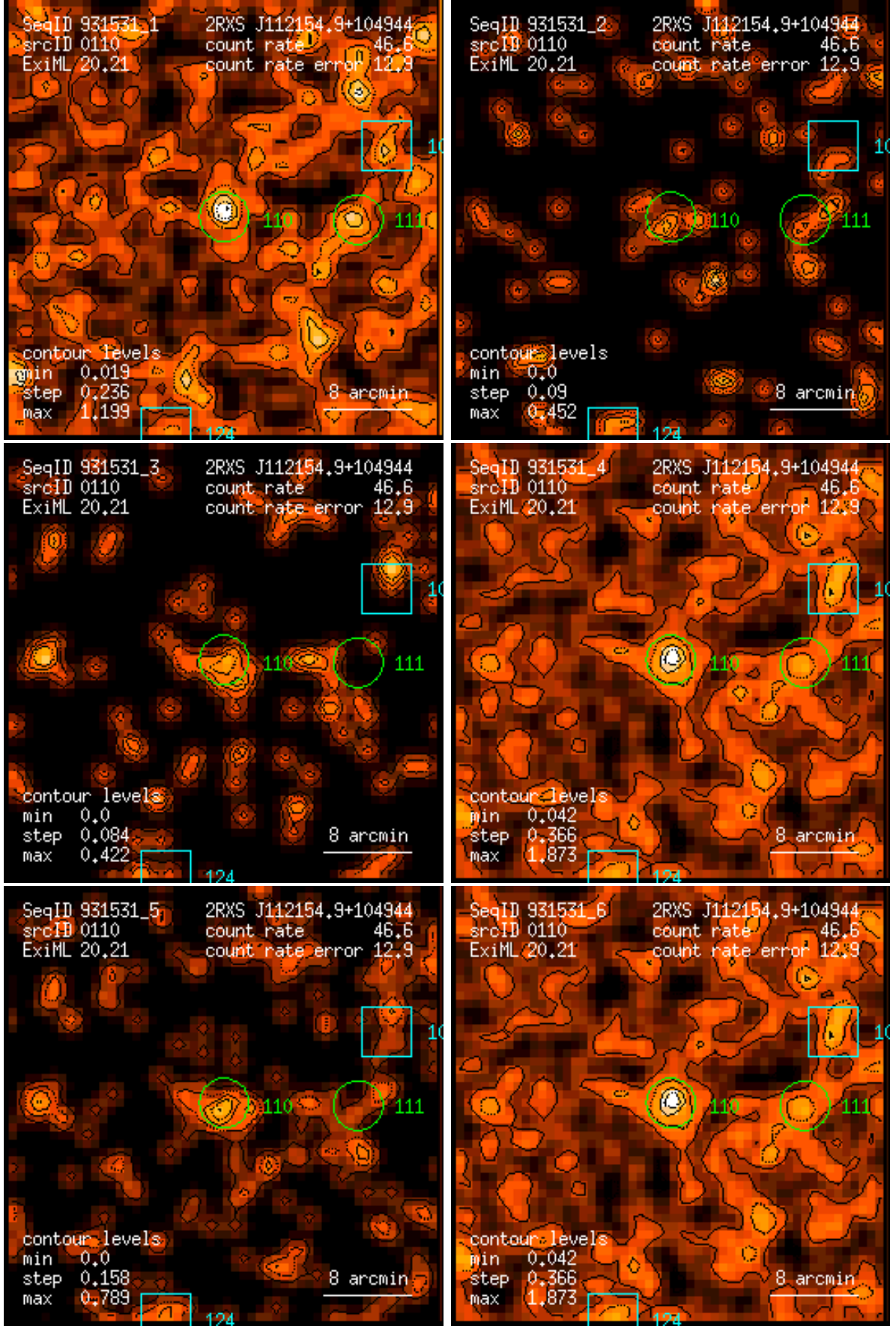
Figure 110: RASS 931531: detection 0110: band rate images, Gaussian filter: (1) PSPC channels 11 – 41, (2) 52 – 90, (3) 91 – 201, (4) 11 – 235, (5) 52 – 201, (6) 11 – 201. Broad band rates in counts/ks. Band rate contour levels in counts/ks/arcmin 2 .
