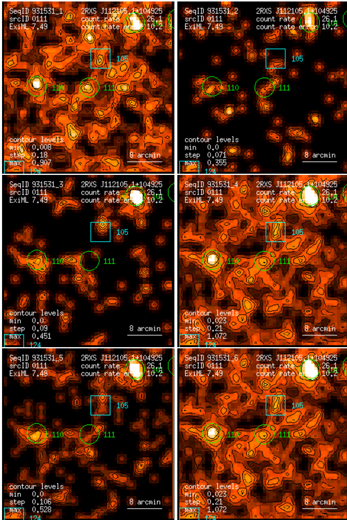
Figure 111: RASS 931531: detection 0111: band rate images, Gaussian filter: (1) PSPC channels 11 – 41, (2) 52 – 90, (3) 91 – 201, (4) 11 – 235, (5) 52 – 201, (6) 11 – 201. Broad band rates in counts/ks. Band rate contour levels in counts/ks/arcmin 2 .
