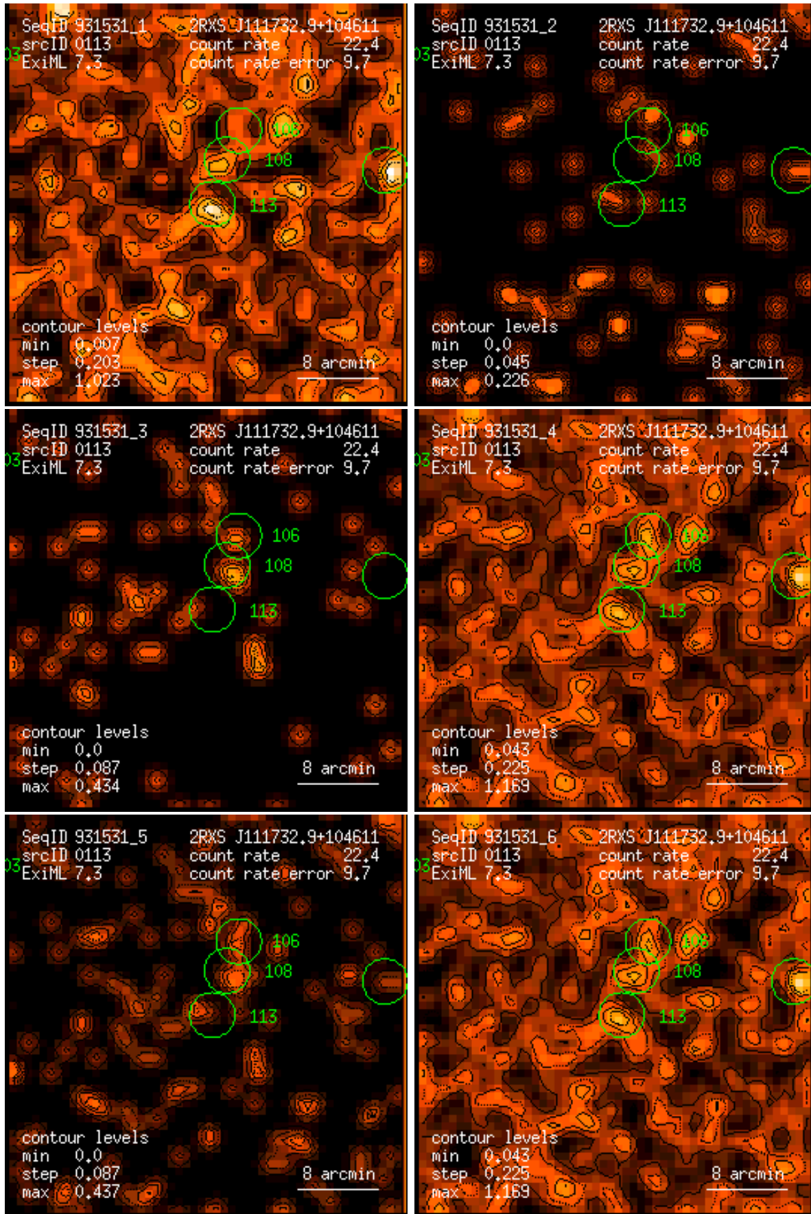
Figure 113: RASS 931531: detection 0113: band rate images, Gaussian filter: (1) PSPC channels 11 – 41, (2) 52 – 90, (3) 91 – 201, (4) 11 – 235, (5) 52 – 201, (6) 11 – 201. Broad band rates in counts/ks. Band rate contour levels in counts/ks/arcmin 2 .
