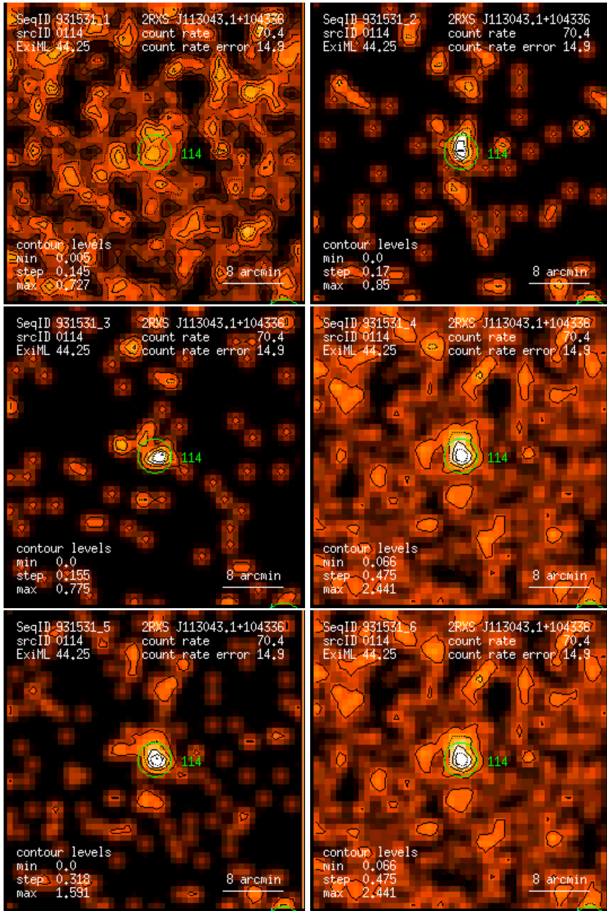
Figure 114: RASS 931531: detection 0114: band rate images, Gaussian filter: (1) PSPC channels 11 – 41, (2) 52 – 90, (3) 91 – 201, (4) 11 – 235, (5) 52 – 201, (6) 11 – 201. Broad band rates in counts/ks. Band rate contour levels in counts/ks/arcmin 2 .
