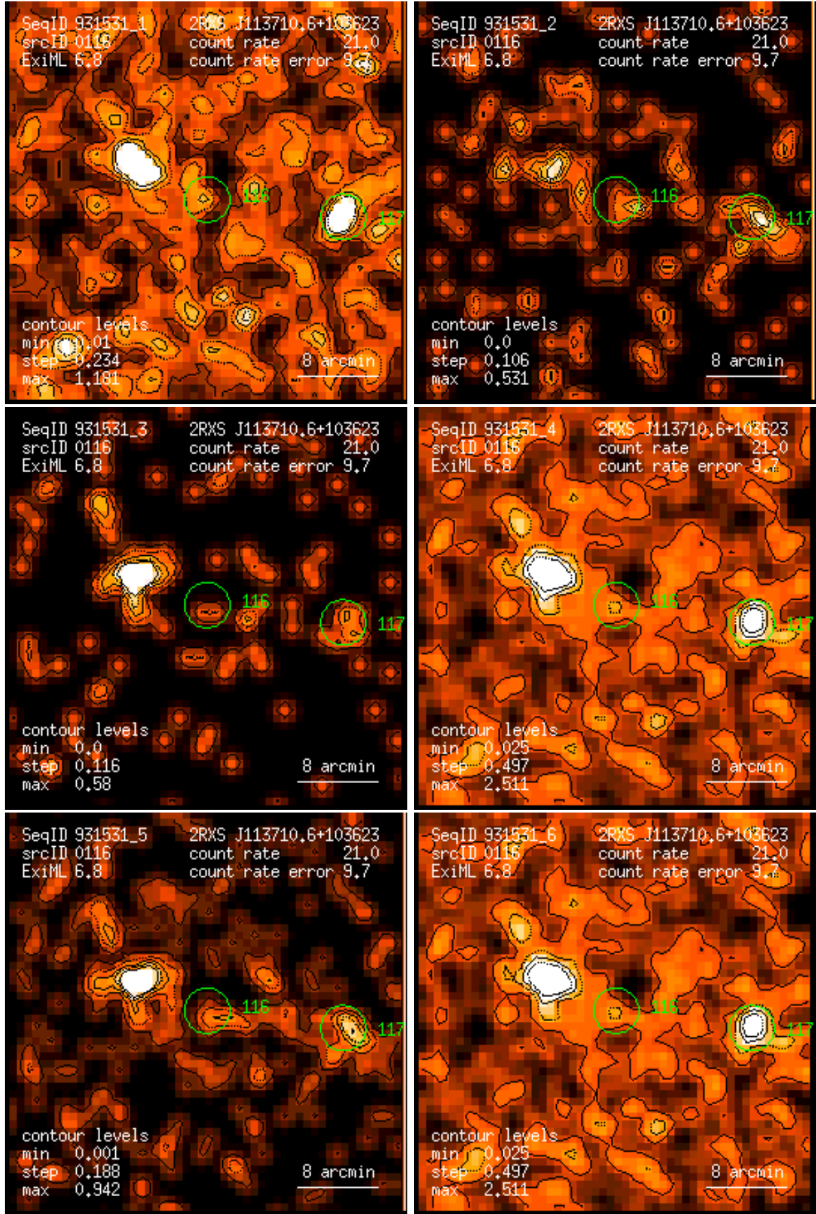
Figure 116: RASS 931531: detection 0116: band rate images, Gaussian filter: (1) PSPC channels 11 – 41, (2) 52 – 90, (3) 91 – 201, (4) 11 – 235, (5) 52 – 201, (6) 11 – 201. Broad band rates in counts/ks. Band rate contour levels in counts/ks/arcmin 2 .
