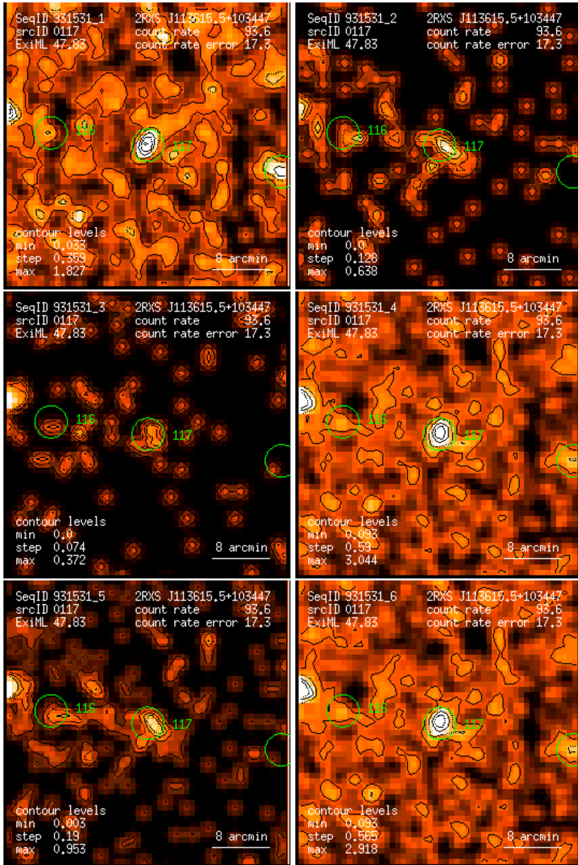
Figure 117: RASS 931531: detection 0117: band rate images, Gaussian filter: (1) PSPC channels 11 – 41, (2) 52 – 90, (3) 91 – 201, (4) 11 – 235, (5) 52 – 201, (6) 11 – 201. Broad band rates in counts/ks. Band rate contour levels in counts/ks/arcmin 2 .
