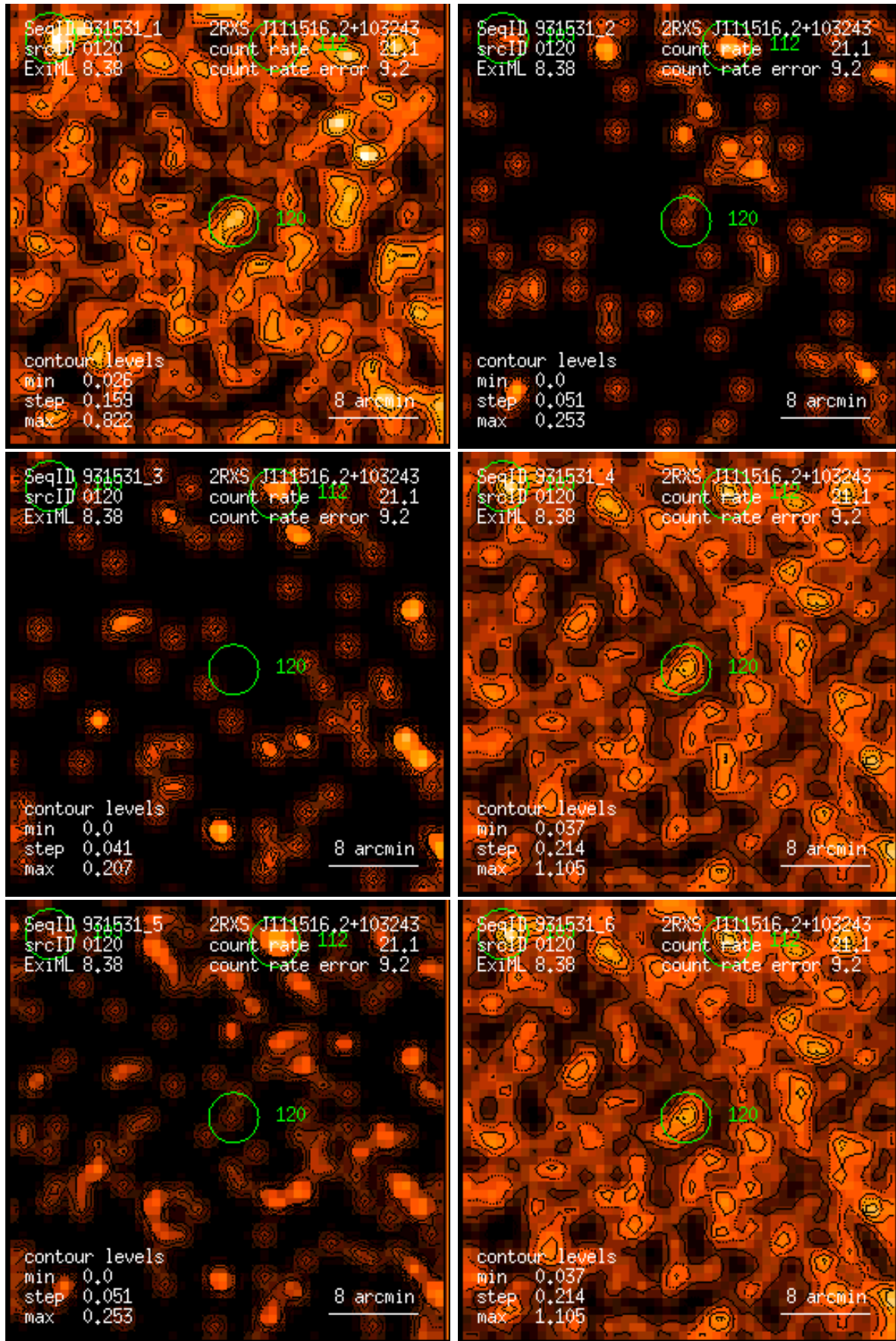
Figure 120: RASS 931531: detection 0120: band rate images, Gaussian filter: (1) PSPC channels 11 – 41, (2) 52 – 90, (3) 91 – 201, (4) 11 – 235, (5) 52 – 201, (6) 11 – 201. Broad band rates in counts/ks. Band rate contour levels in counts/ks/arcmin 2 .
