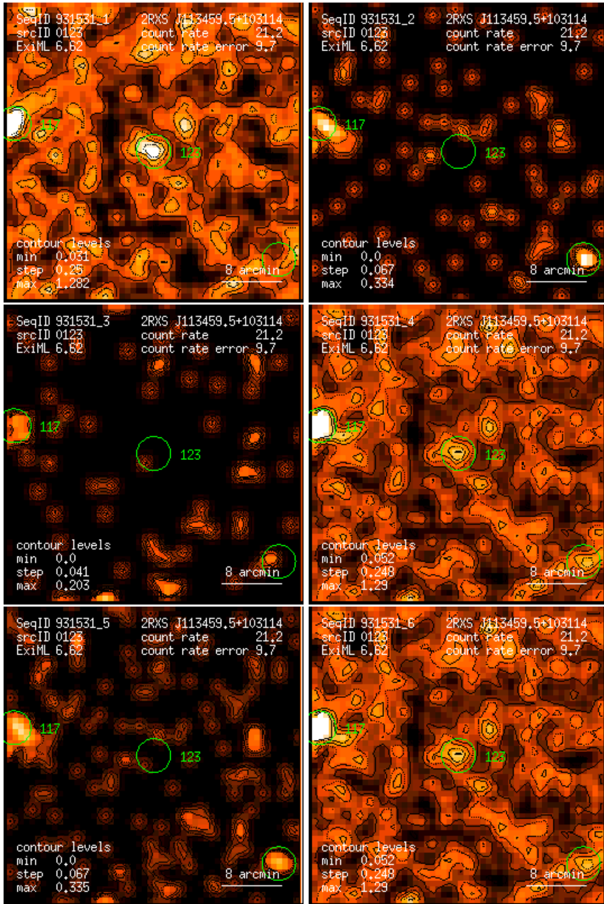
Figure 123: RASS 931531: detection 0123: band rate images, Gaussian filter: (1) PSPC channels 11 – 41, (2) 52 – 90, (3) 91 – 201, (4) 11 – 235, (5) 52 – 201, (6) 11 – 201. Broad band rates in counts/ks. Band rate contour levels in counts/ks/arcmin 2 .
