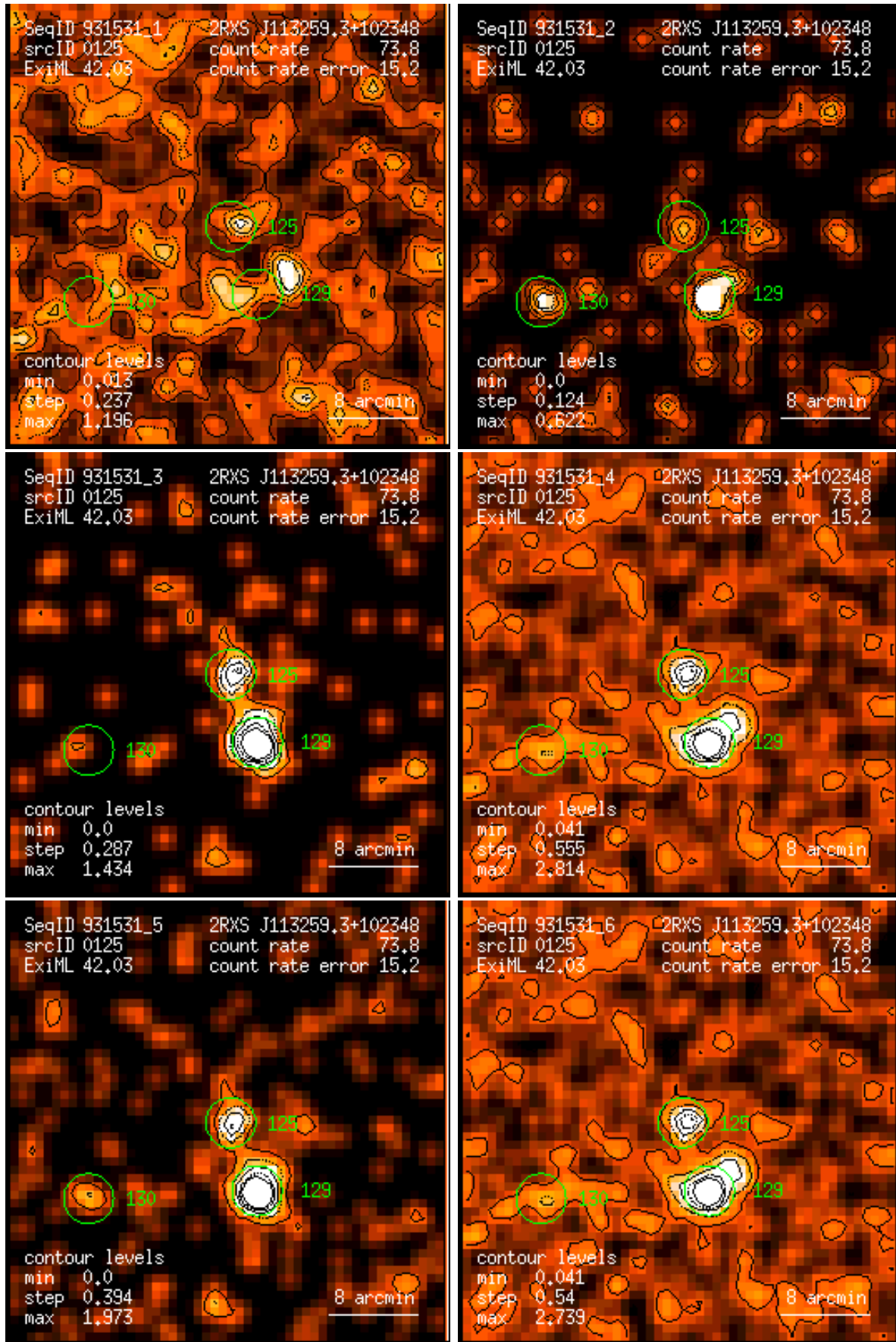
Figure 125: RASS 931531: detection 0125: band rate images, Gaussian filter: (1) PSPC channels 11 – 41, (2) 52 – 90, (3) 91 – 201, (4) 11 – 235, (5) 52 – 201, (6) 11 – 201. Broad band rates in counts/ks. Band rate contour levels in counts/ks/arcmin 2 .
