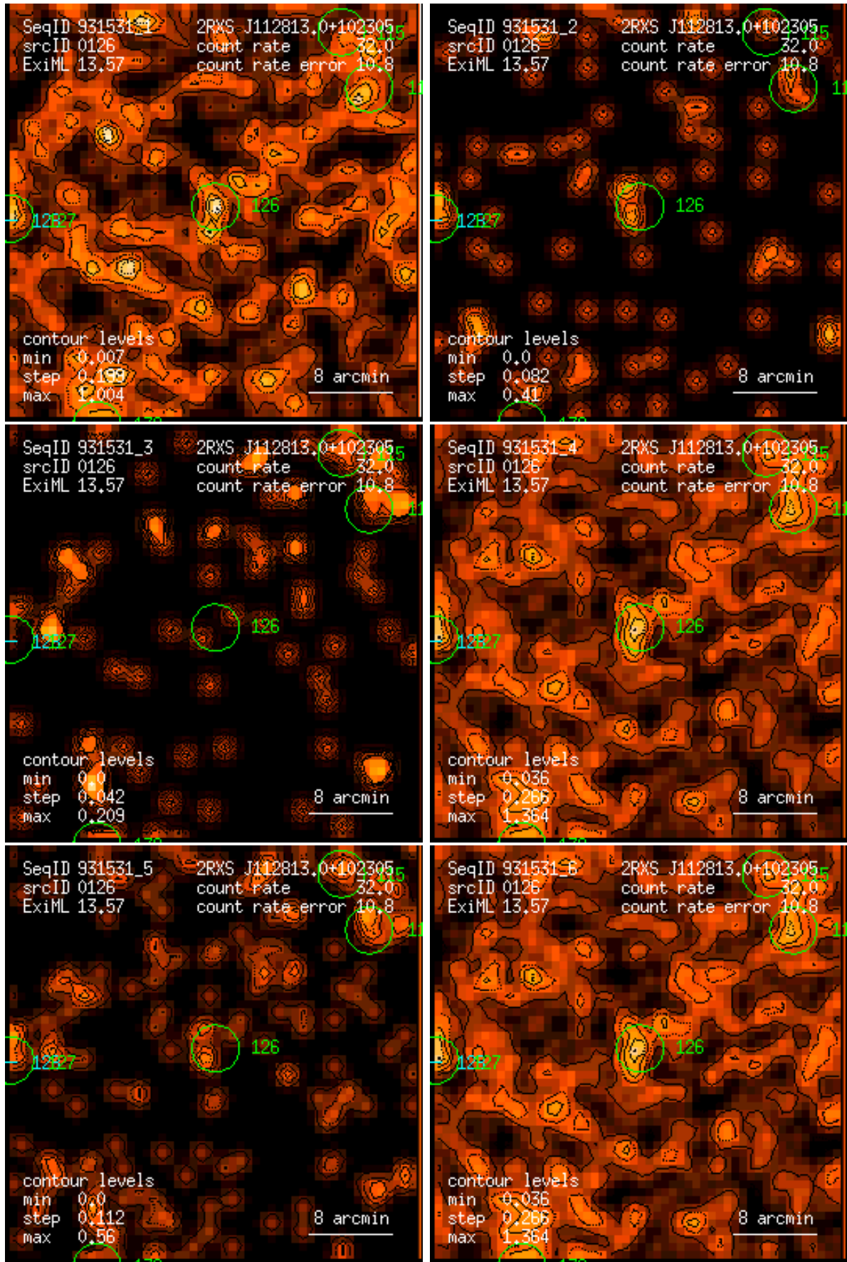
Figure 126: RASS 931531: detection 0126: band rate images, Gaussian filter: (1) PSPC channels 11 – 41, (2) 52 – 90, (3) 91 – 201, (4) 11 – 235, (5) 52 – 201, (6) 11 – 201. Broad band rates in counts/ks. Band rate contour levels in counts/ks/arcmin 2 .
