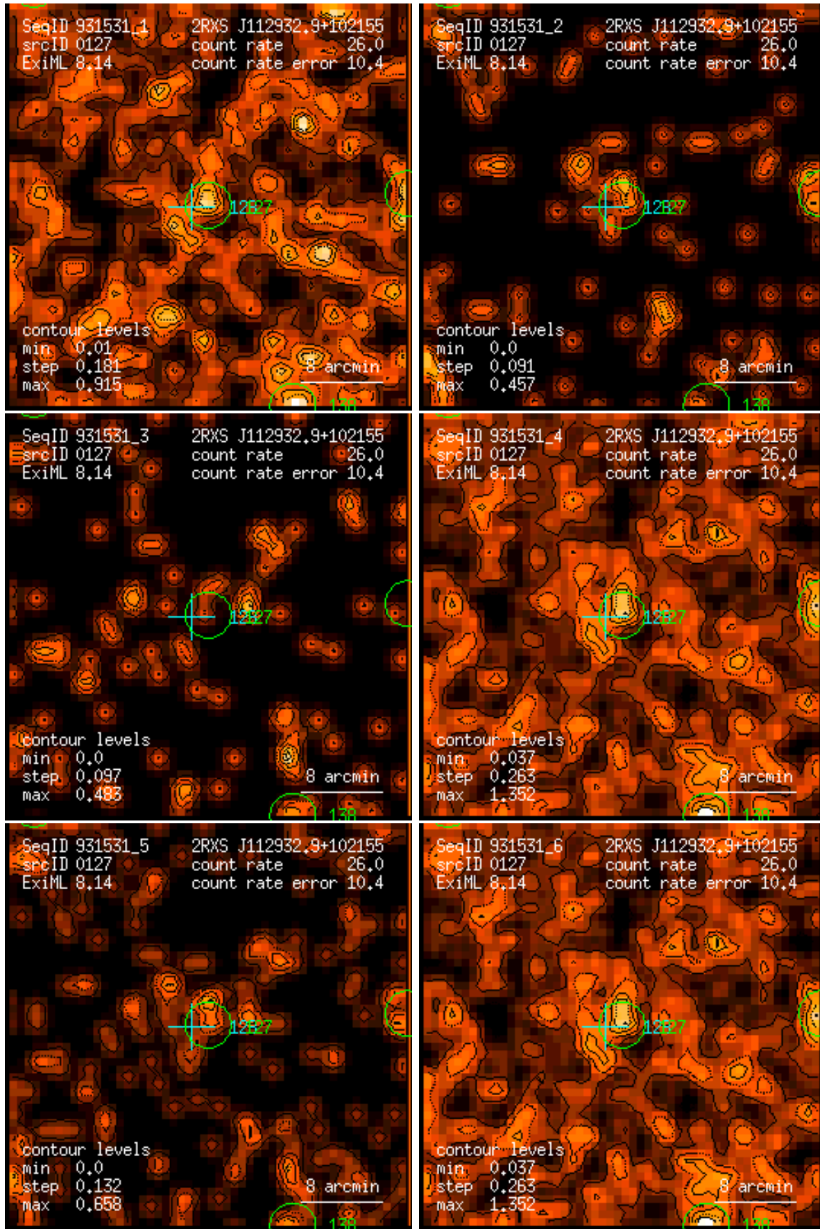
Figure 127: RASS 931531: detection 0127: band rate images, Gaussian filter: (1) PSPC channels 11 – 41, (2) 52 – 90, (3) 91 – 201, (4) 11 – 235, (5) 52 – 201, (6) 11 – 201. Broad band rates in counts/ks. Band rate contour levels in counts/ks/arcmin 2 .
