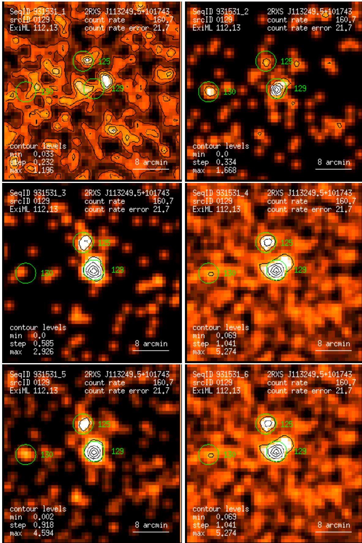
Figure 129: RASS 931531: detection 0129: band rate images, Gaussian filter: (1) PSPC channels 11 – 41, (2) 52 – 90, (3) 91 – 201, (4) 11 – 235, (5) 52 – 201, (6) 11 – 201. Broad band rates in counts/ks. Band rate contour levels in counts/ks/arcmin 2 .
