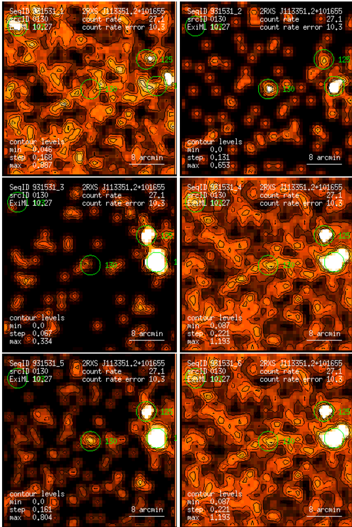
Figure 130: RASS 931531: detection 0130: band rate images, Gaussian filter: (1) PSPC channels 11 – 41, (2) 52 – 90, (3) 91 – 201, (4) 11 – 235, (5) 52 – 201, (6) 11 – 201. Broad band rates in counts/ks. Band rate contour levels in counts/ks/arcmin 2 .
