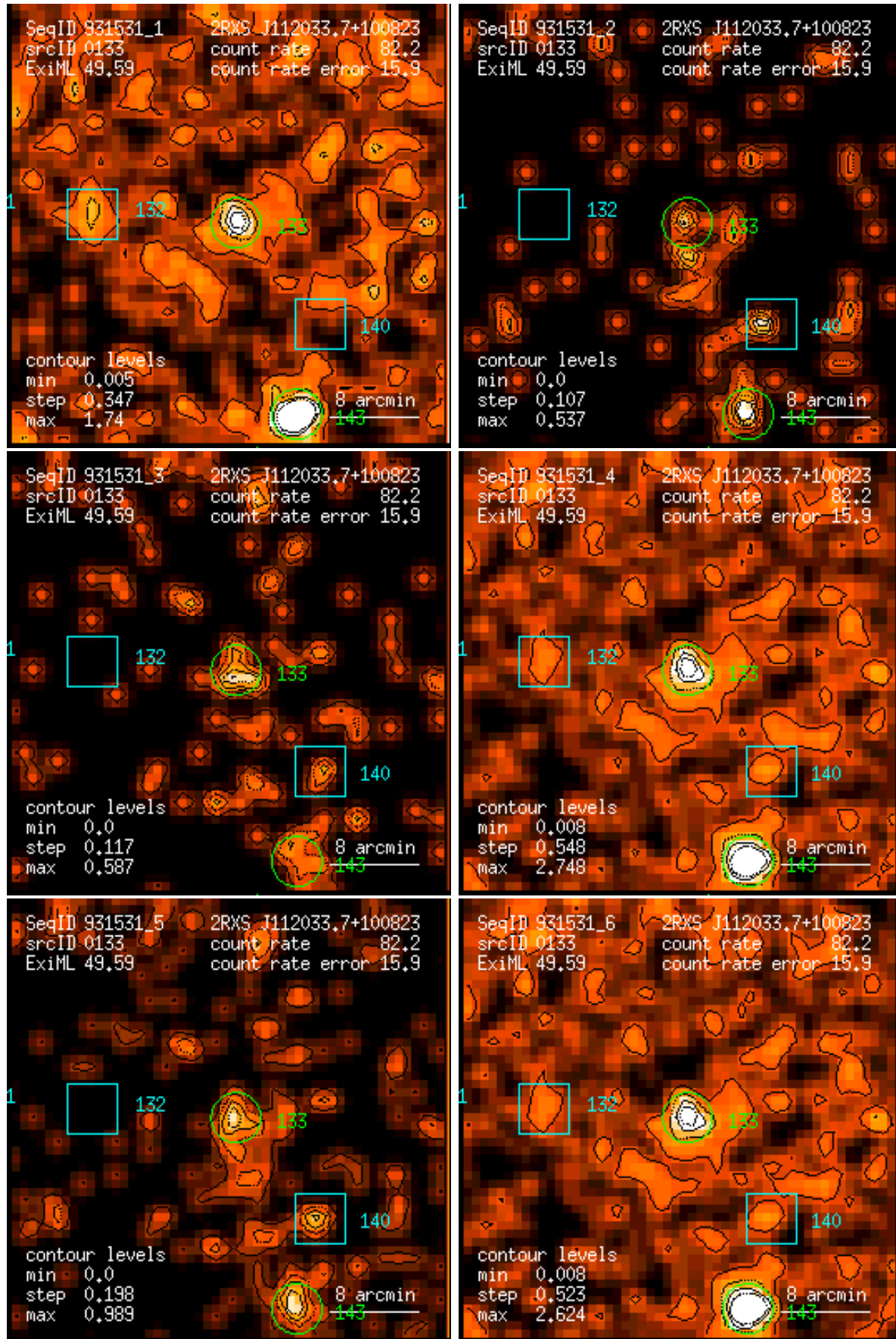
Figure 133: RASS 931531: detection 0133: band rate images, Gaussian filter: (1) PSPC channels 11 – 41, (2) 52 – 90, (3) 91 – 201, (4) 11 – 235, (5) 52 – 201, (6) 11 – 201. Broad band rates in counts/ks. Band rate contour levels in counts/ks/arcmin 2 .
