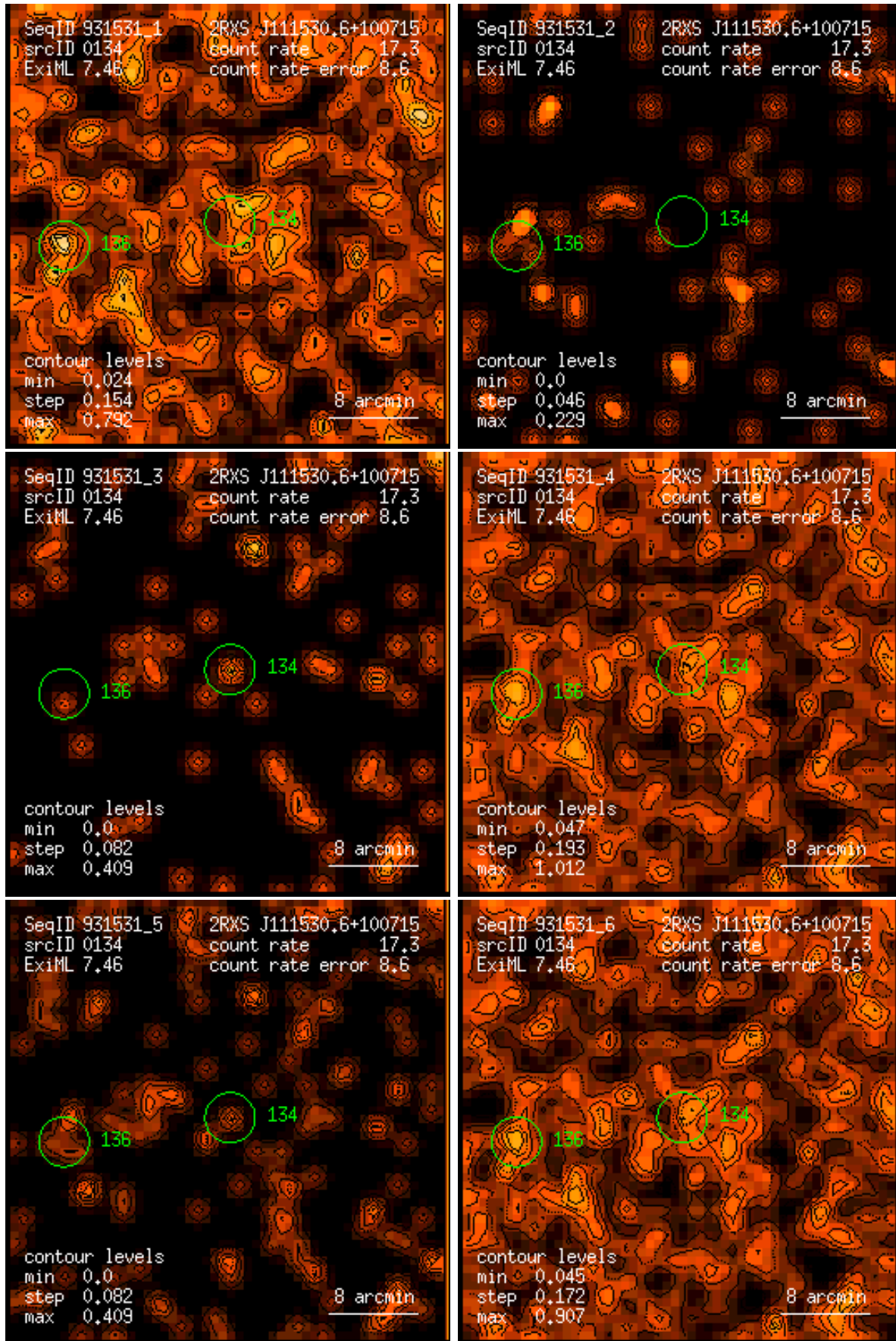
Figure 134: RASS 931531: detection 0134: band rate images, Gaussian filter: (1) PSPC channels 11 – 41, (2) 52 – 90, (3) 91 – 201, (4) 11 – 235, (5) 52 – 201, (6) 11 – 201. Broad band rates in counts/ks. Band rate contour levels in counts/ks/arcmin 2 .
