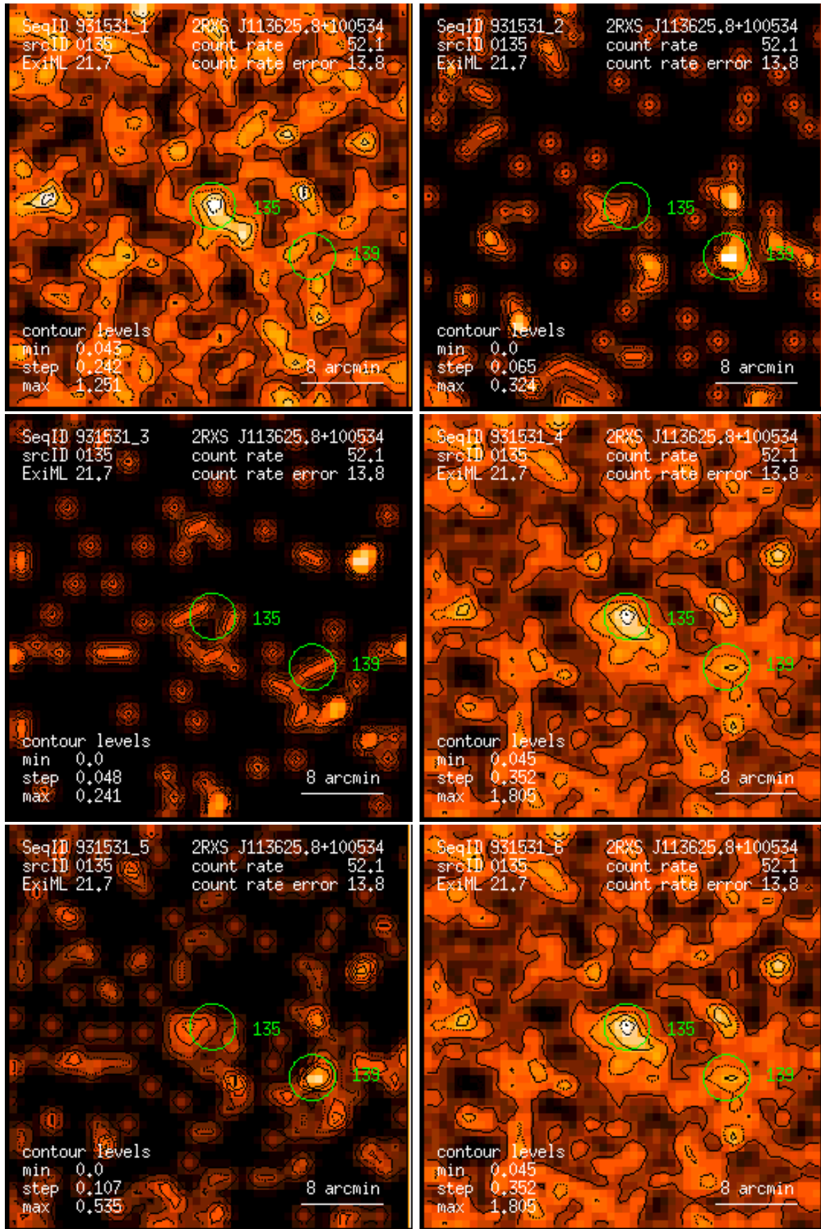
Figure 135: RASS 931531: detection 0135: band rate images, Gaussian filter: (1) PSPC channels 11 – 41, (2) 52 – 90, (3) 91 – 201, (4) 11 – 235, (5) 52 – 201, (6) 11 – 201. Broad band rates in counts/ks. Band rate contour levels in counts/ks/arcmin 2 .
