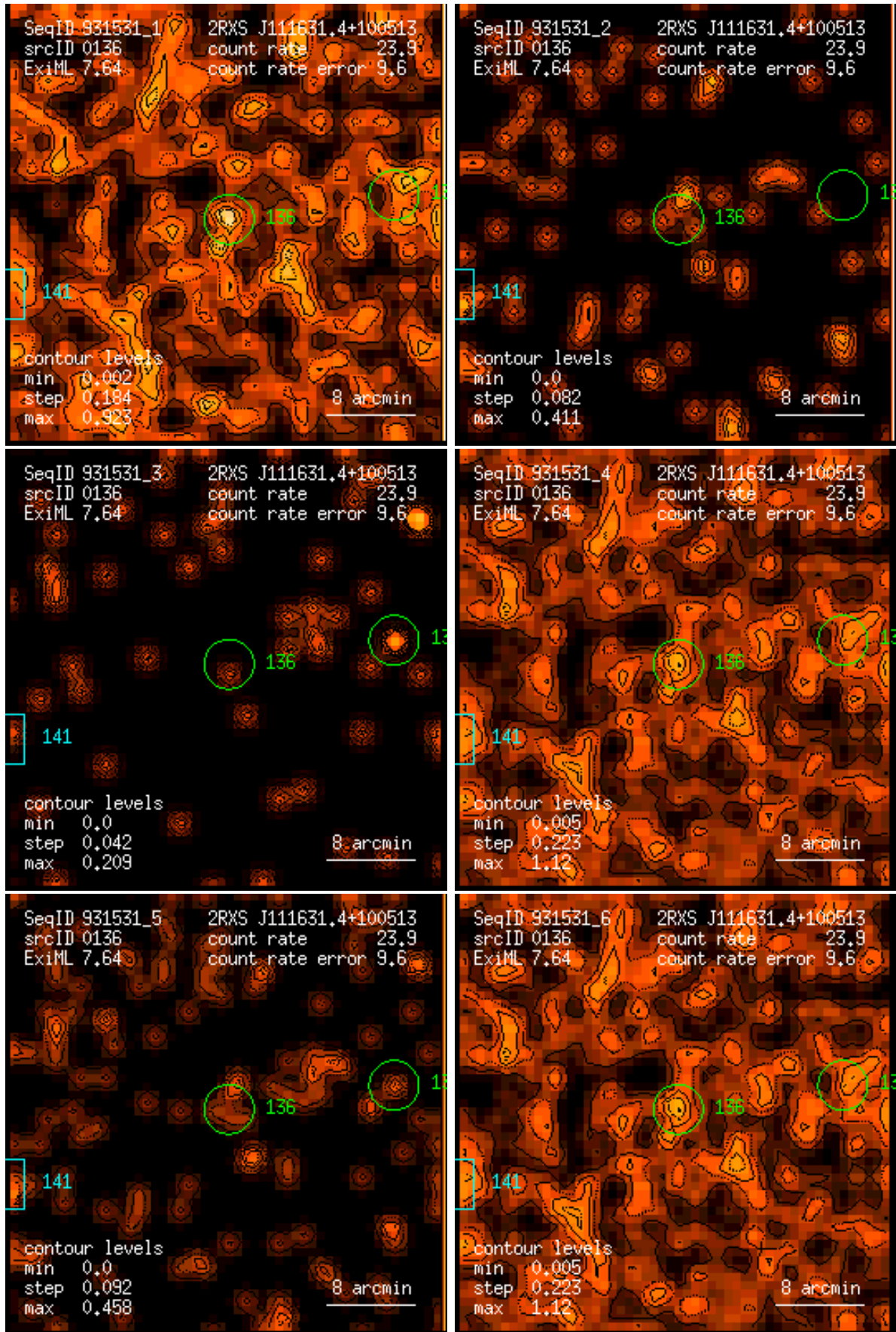
Figure 136: RASS 931531: detection 0136: band rate images, Gaussian filter: (1) PSPC channels 11 – 41, (2) 52 – 90, (3) 91 – 201, (4) 11 – 235, (5) 52 – 201, (6) 11 – 201. Broad band rates in counts/ks. Band rate contour levels in counts/ks/arcmin 2 .
