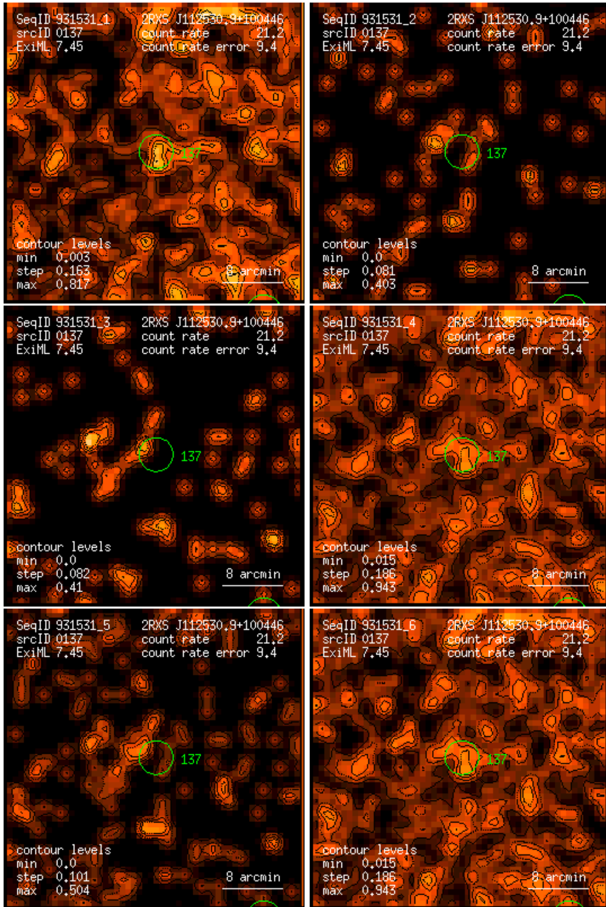
Figure 137: RASS 931531: detection 0137: band rate images, Gaussian filter: (1) PSPC channels 11 – 41, (2) 52 – 90, (3) 91 – 201, (4) 11 – 235, (5) 52 – 201, (6) 11 – 201. Broad band rates in counts/ks. Band rate contour levels in counts/ks/arcmin 2 .
