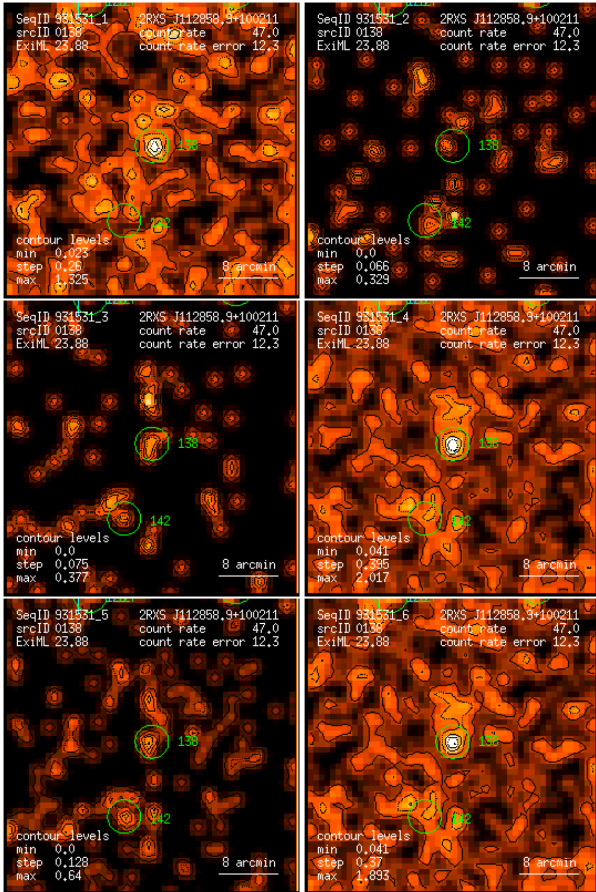
Figure 138: RASS 931531: detection 0138: band rate images, Gaussian filter: (1) PSPC channels 11 – 41, (2) 52 – 90, (3) 91 – 201, (4) 11 – 235, (5) 52 – 201, (6) 11 – 201. Broad band rates in counts/ks. Band rate contour levels in counts/ks/arcmin 2 .
