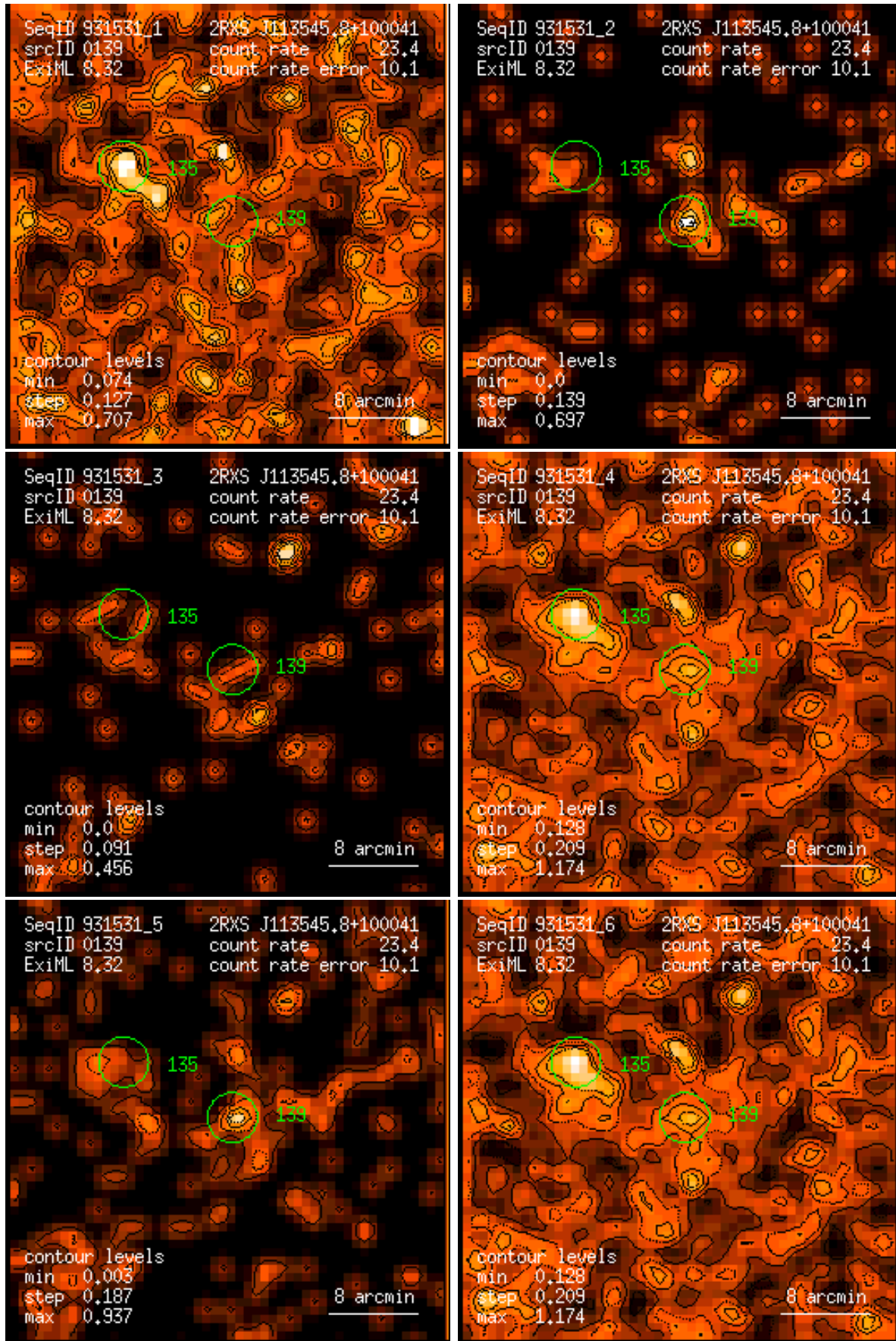
Figure 139: RASS 931531: detection 0139: band rate images, Gaussian filter: (1) PSPC channels 11 – 41, (2) 52 – 90, (3) 91 – 201, (4) 11 – 235, (5) 52 – 201, (6) 11 – 201. Broad band rates in counts/ks. Band rate contour levels in counts/ks/arcmin 2 .
