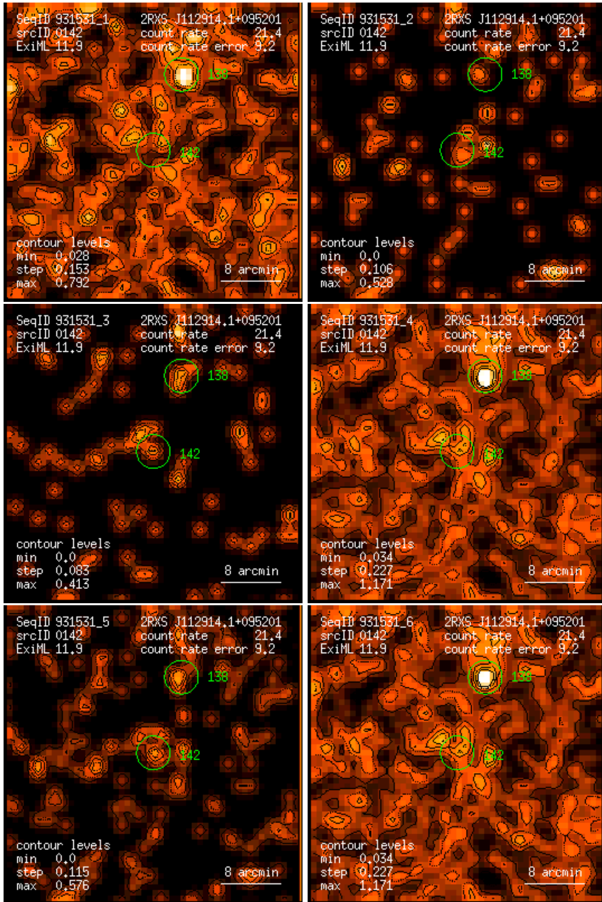
Figure 142: RASS 931531: detection 0142: band rate images, Gaussian filter: (1) PSPC channels 11 – 41, (2) 52 – 90, (3) 91 – 201, (4) 11 – 235, (5) 52 – 201, (6) 11 – 201. Broad band rates in counts/ks. Band rate contour levels in counts/ks/arcmin 2 .
