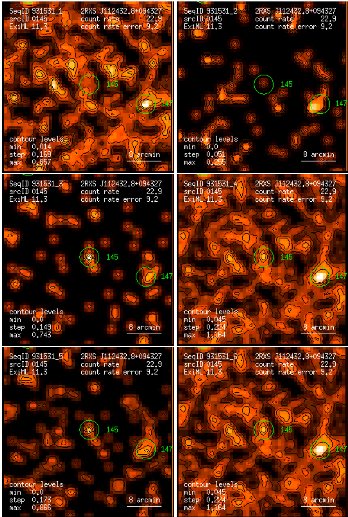
Figure 145: RASS 931531: detection 0145: band rate images, Gaussian filter: (1) PSPC channels 11 – 41, (2) 52 – 90, (3) 91 – 201, (4) 11 – 235, (5) 52 – 201, (6) 11 – 201. Broad band rates in counts/ks. Band rate contour levels in counts/ks/arcmin 2 .
