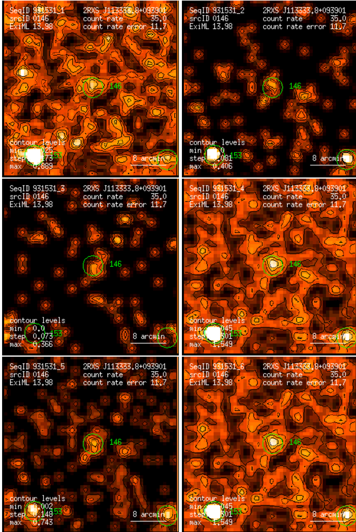
Figure 146: RASS 931531: detection 0146: band rate images, Gaussian filter: (1) PSPC channels 11 – 41, (2) 52 – 90, (3) 91 – 201, (4) 11 – 235, (5) 52 – 201, (6) 11 – 201. Broad band rates in counts/ks. Band rate contour levels in counts/ks/arcmin 2 .
