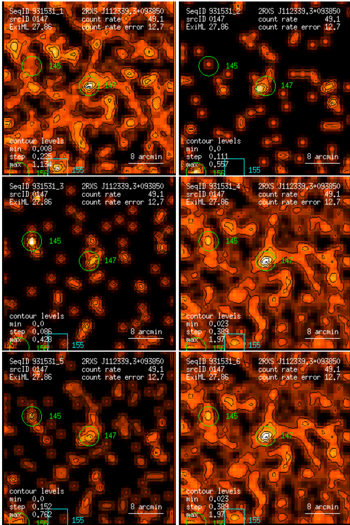
Figure 147: RASS 931531: detection 0147: band rate images, Gaussian filter: (1) PSPC channels 11 – 41, (2) 52 – 90, (3) 91 – 201, (4) 11 – 235, (5) 52 – 201, (6) 11 – 201. Broad band rates in counts/ks. Band rate contour levels in counts/ks/arcmin 2 .
