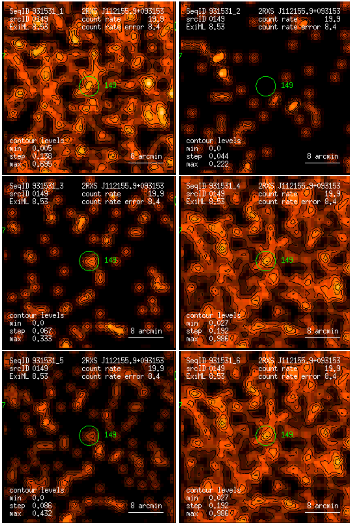
Figure 149: RASS 931531: detection 0149: band rate images, Gaussian filter: (1) PSPC channels 11 – 41, (2) 52 – 90, (3) 91 – 201, (4) 11 – 235, (5) 52 – 201, (6) 11 – 201. Broad band rates in counts/ks. Band rate contour levels in counts/ks/arcmin 2 .
