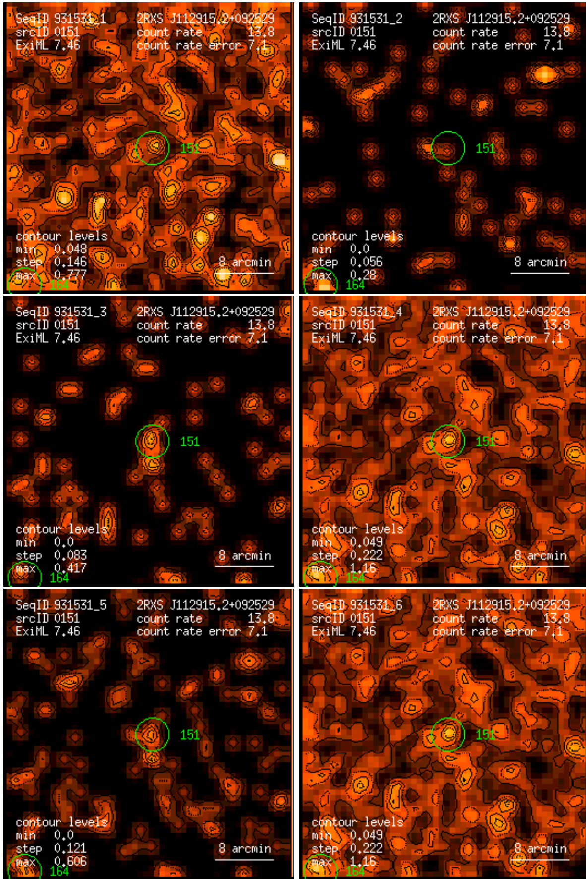
Figure 151: RASS 931531: detection 0151: band rate images, Gaussian filter: (1) PSPC channels 11 – 41, (2) 52 – 90, (3) 91 – 201, (4) 11 – 235, (5) 52 – 201, (6) 11 – 201. Broad band rates in counts/ks. Band rate contour levels in counts/ks/arcmin 2 .
