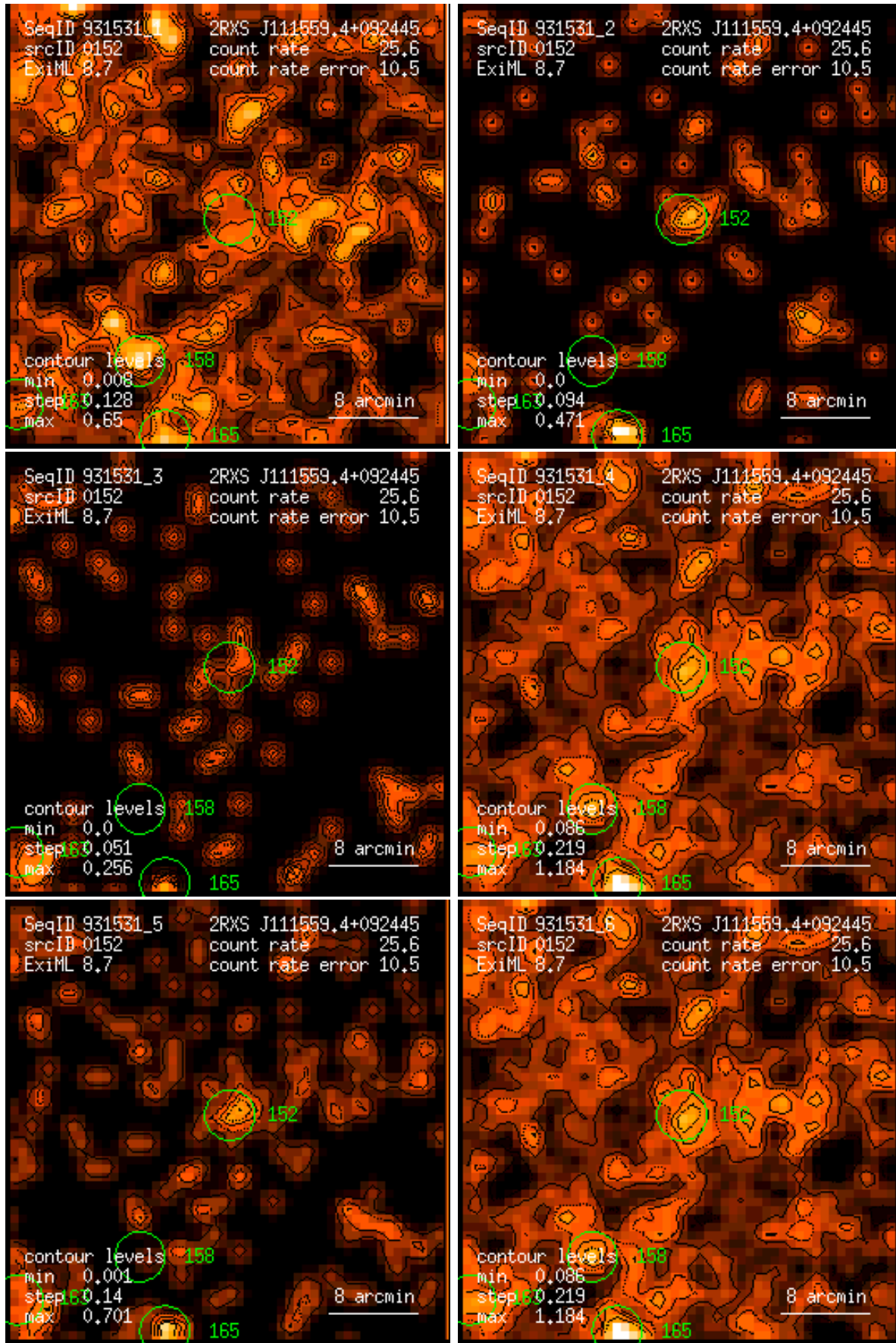
Figure 152: RASS 931531: detection 0152: band rate images, Gaussian filter: (1) PSPC channels 11 – 41, (2) 52 – 90, (3) 91 – 201, (4) 11 – 235, (5) 52 – 201, (6) 11 – 201. Broad band rates in counts/ks. Band rate contour levels in counts/ks/arcmin 2 .
