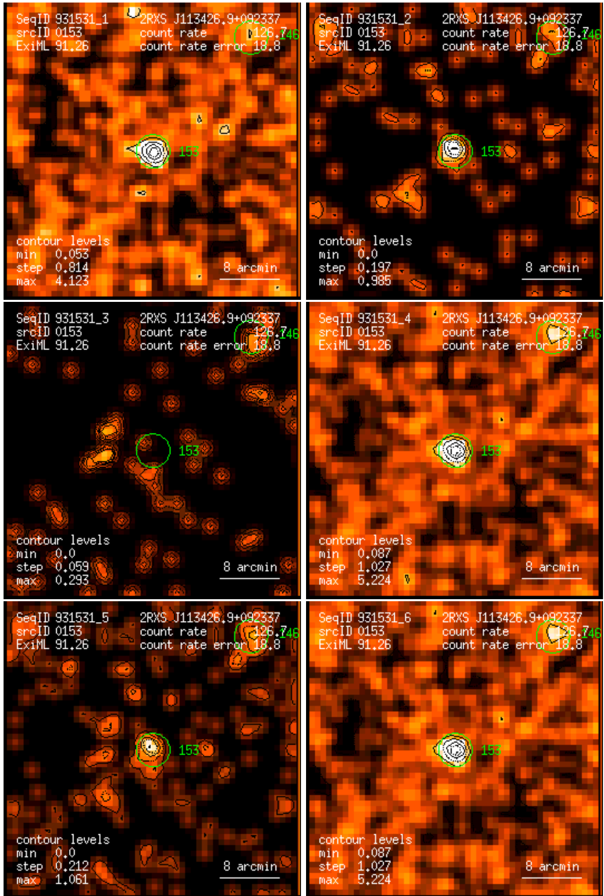
Figure 153: RASS 931531: detection 0153: band rate images, Gaussian filter: (1) PSPC channels 11 – 41, (2) 52 – 90, (3) 91 – 201, (4) 11 – 235, (5) 52 – 201, (6) 11 – 201. Broad band rates in counts/ks. Band rate contour levels in counts/ks/arcmin 2 .
