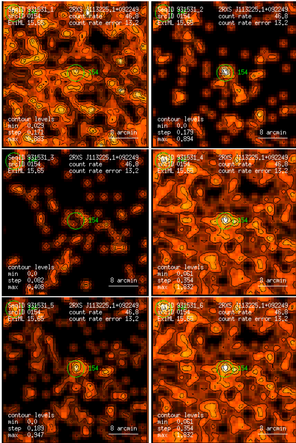
Figure 154: RASS 931531: detection 0154: band rate images, Gaussian filter: (1) PSPC channels 11 – 41, (2) 52 – 90, (3) 91 – 201, (4) 11 – 235, (5) 52 – 201, (6) 11 – 201. Broad band rates in counts/ks. Band rate contour levels in counts/ks/arcmin 2 .
